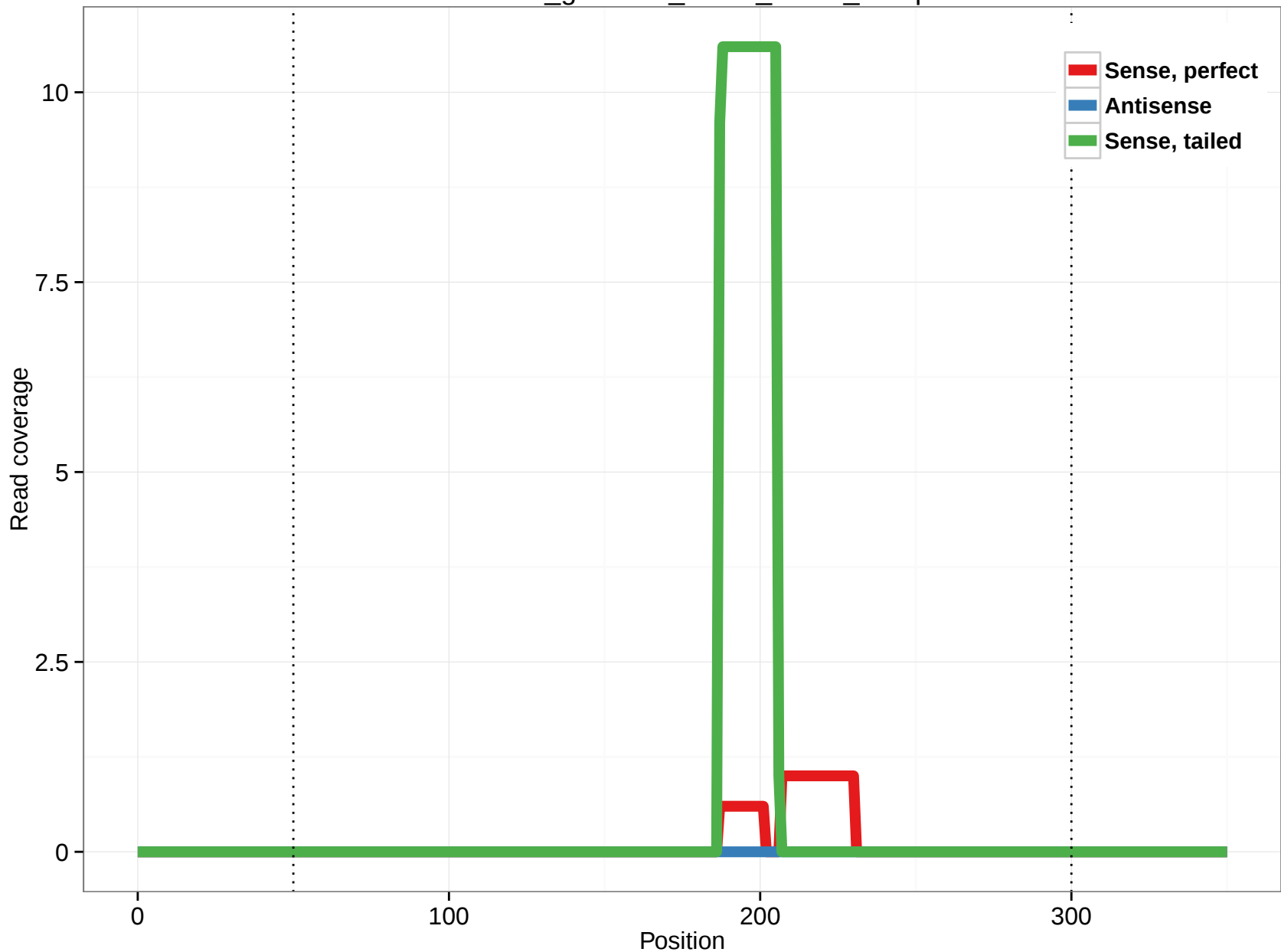
rheMac3_genscan_chr13_32.56_13.5p
