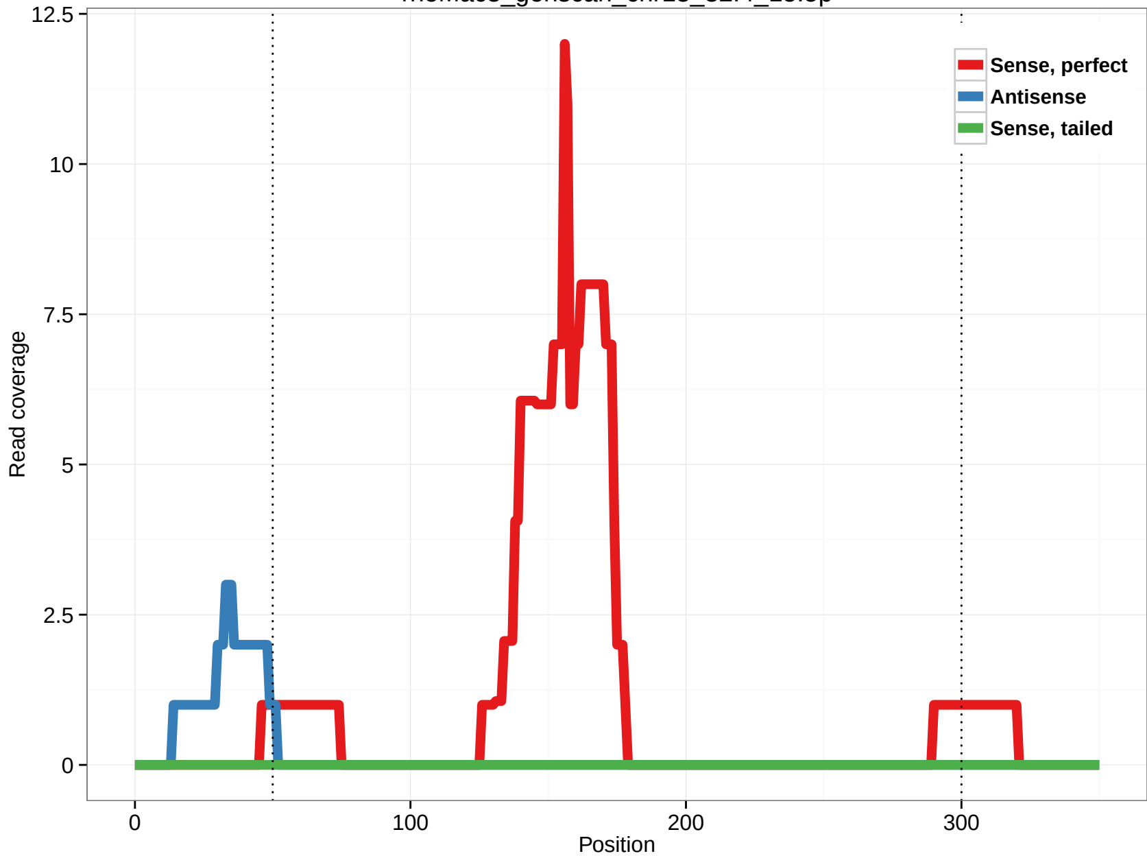
rheMac3_genscan_chr13_32.4_15.5p
