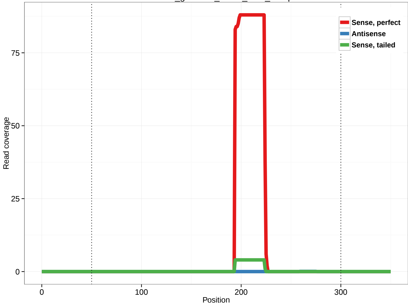
rheMac3_genscan_chr13_32.1_29.5p
