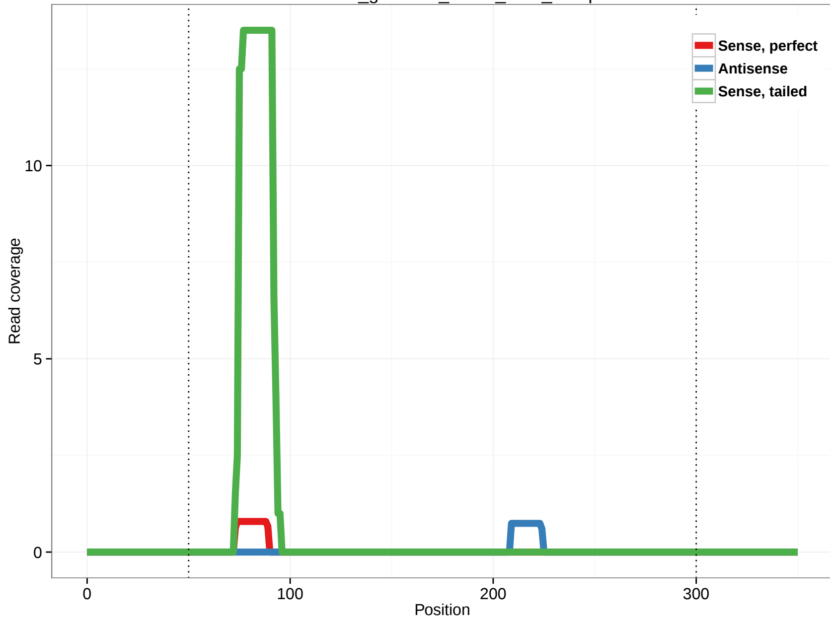
rheMac3_genscan_chr13_24.5_12.3p
