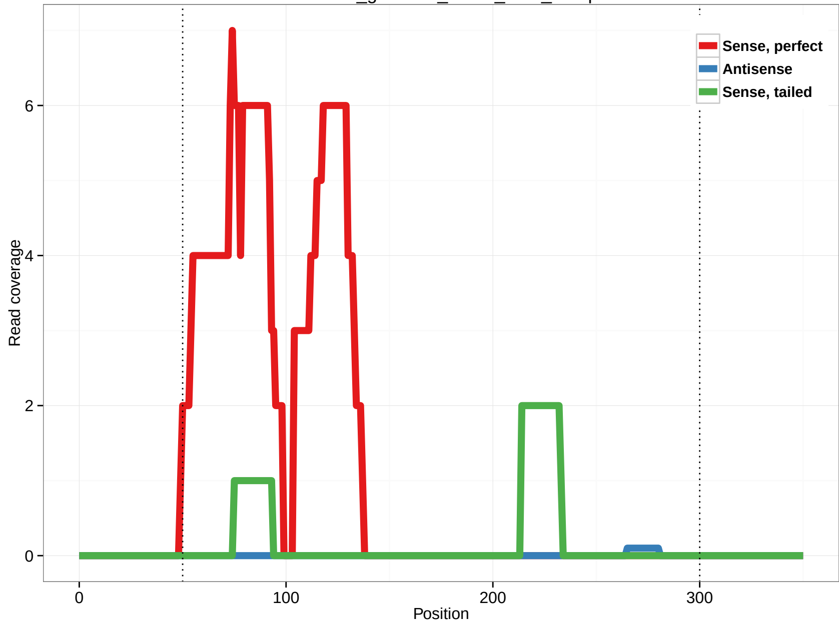
rheMac3_genscan_chr13_24.3_12.5p
