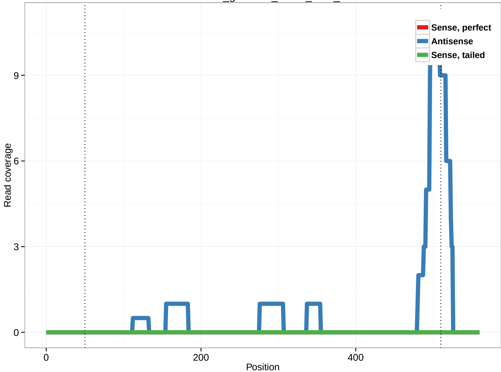
rheMac3_genscan_chr13_22.8_4
