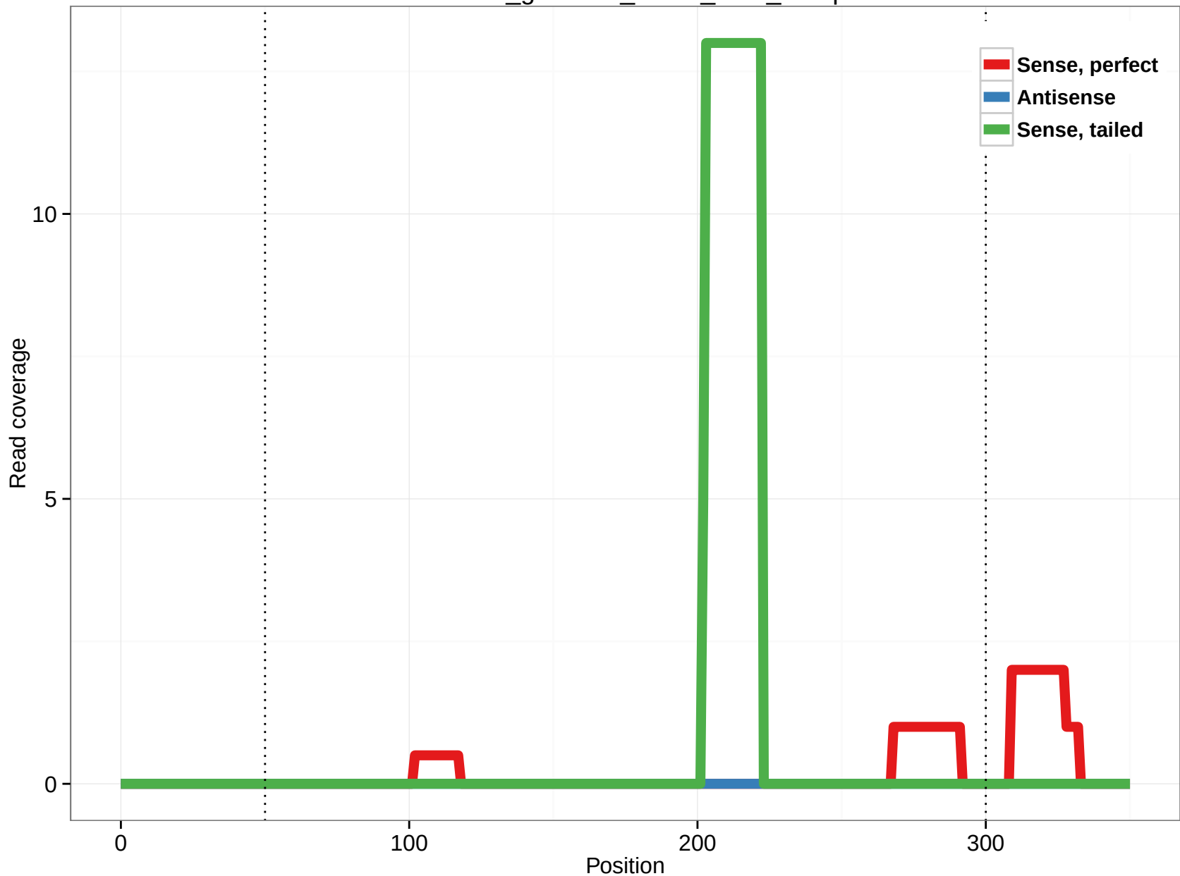
rheMac3_genscan_chr13_22.5_21.3p
