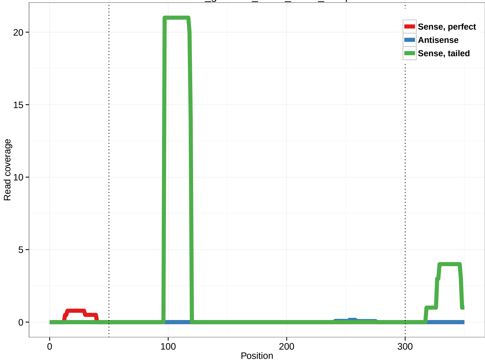
rheMac3_genscan_chr13_22.28_10.5p
