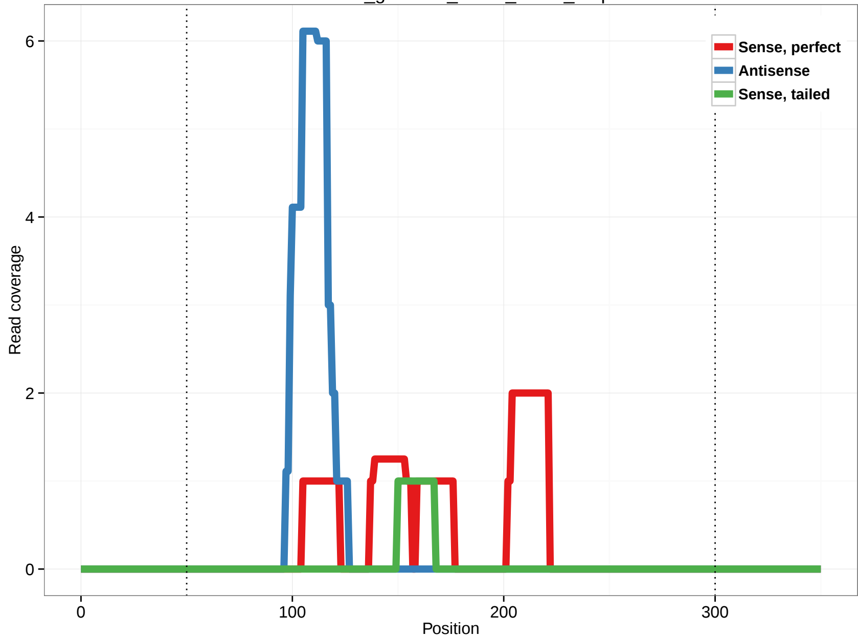
rheMac3_genscan_chr13_22.23_4.3p
