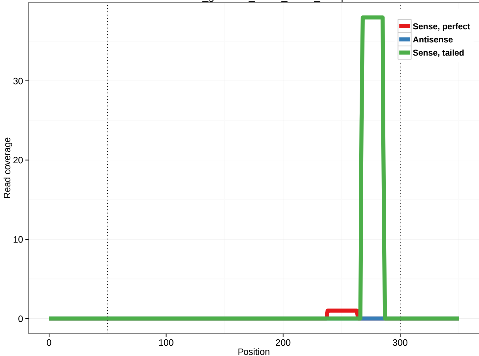
rheMac3_genscan_chr13_22.23_30.5p
