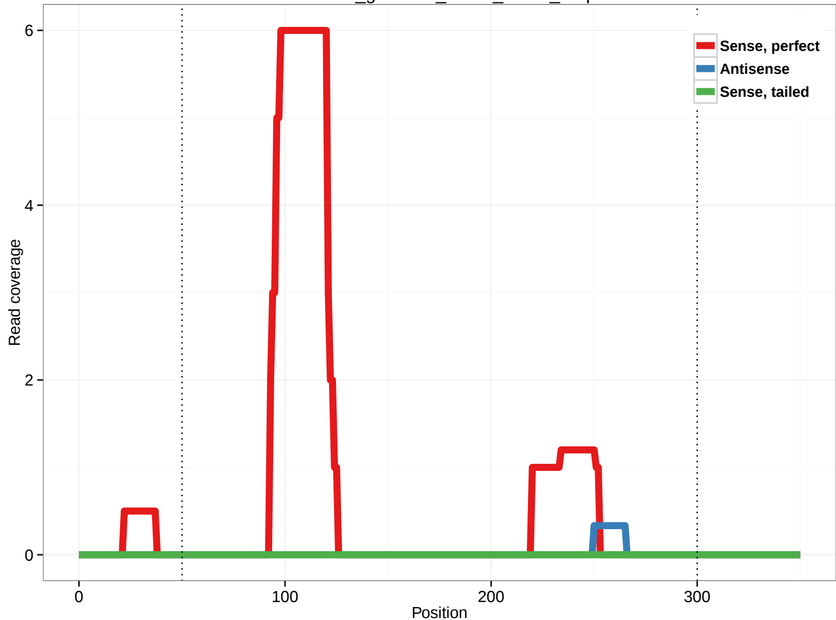
rheMac3_genscan_chr13_22.19_2.3p
