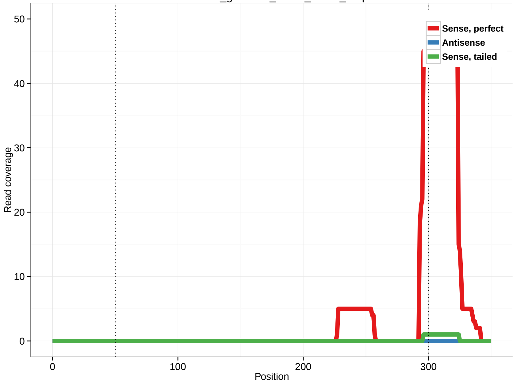
rheMac3_genscan_chr13_22.16_3.3p
