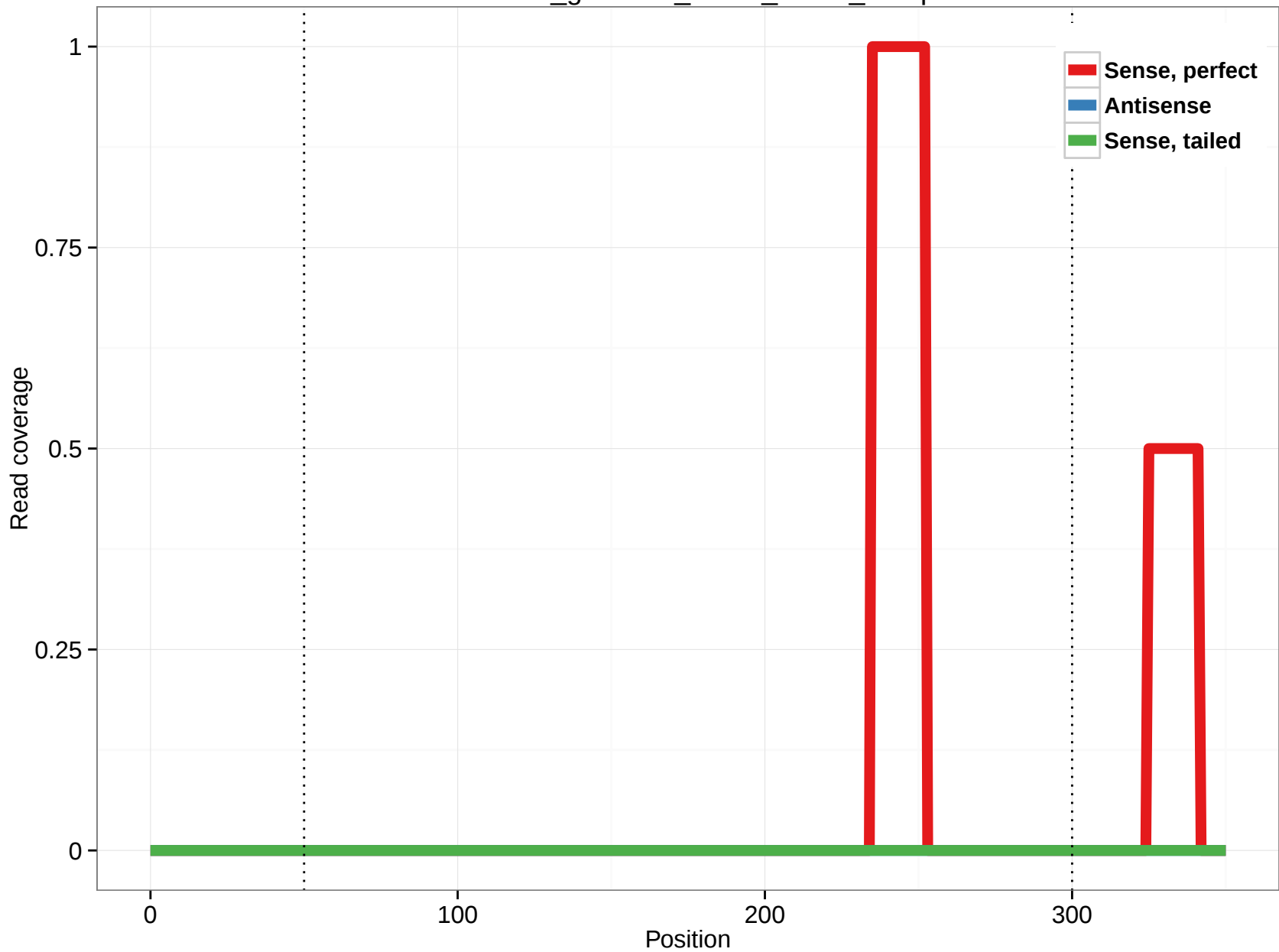
rheMac3_genscan_chr13_22.13_33.3p
