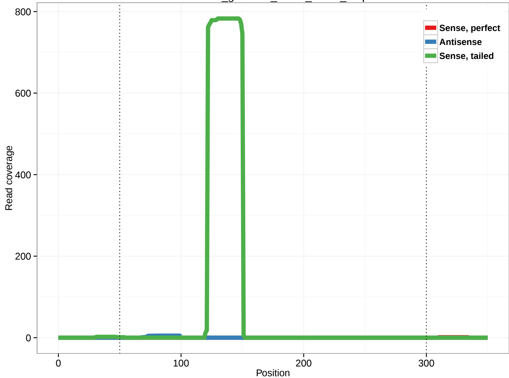
rheMac3_genscan_chr13_22.13_3.3p
