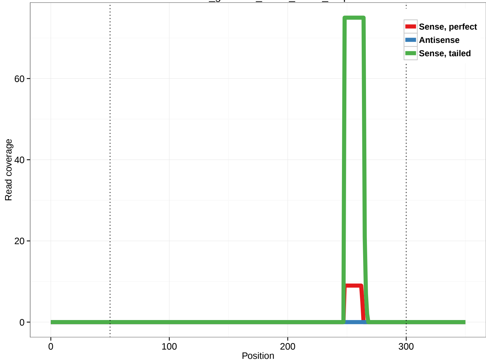
rheMac3_genscan_chr13_22.12_2.3p
