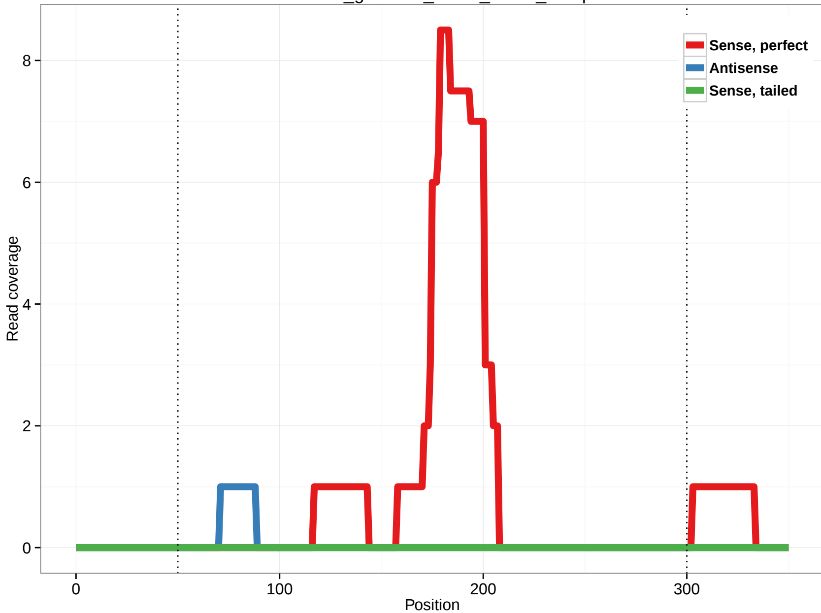
rheMac3_genscan_chr13_214.7_13.5p
