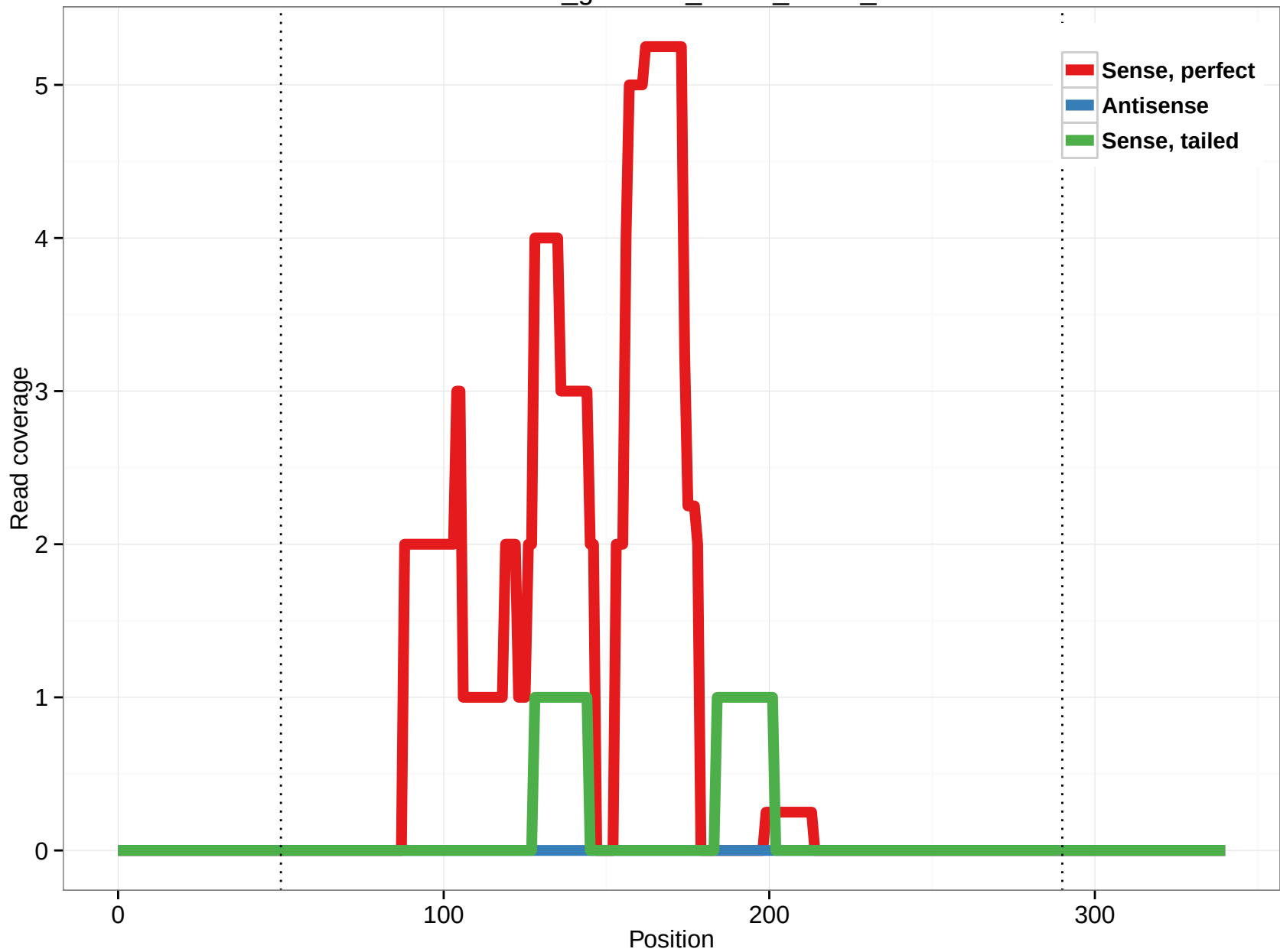
rheMac3_genscan_chr13_214.5_0
