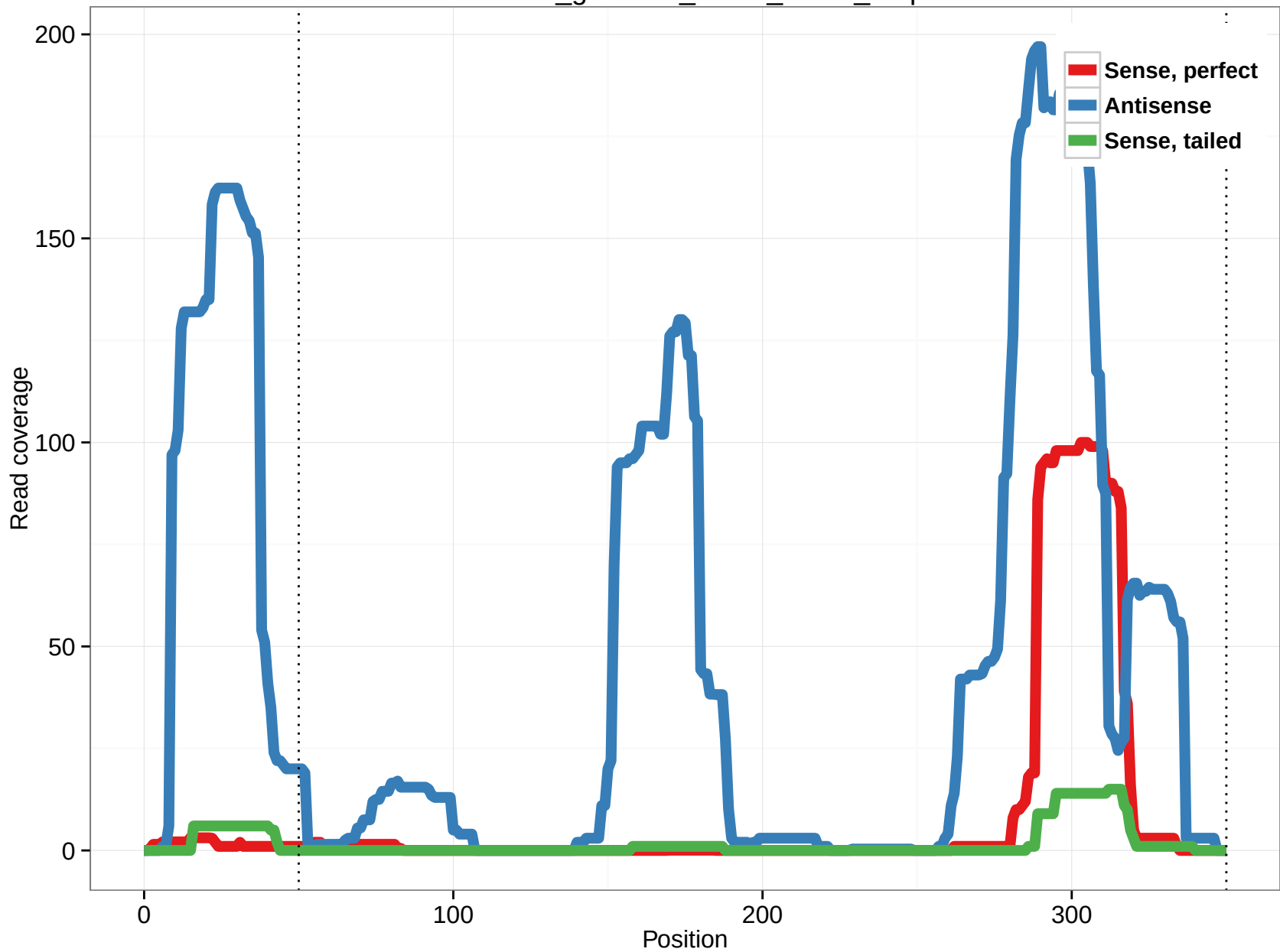
rheMac3_genscan_chr13_213.1_0.5p
