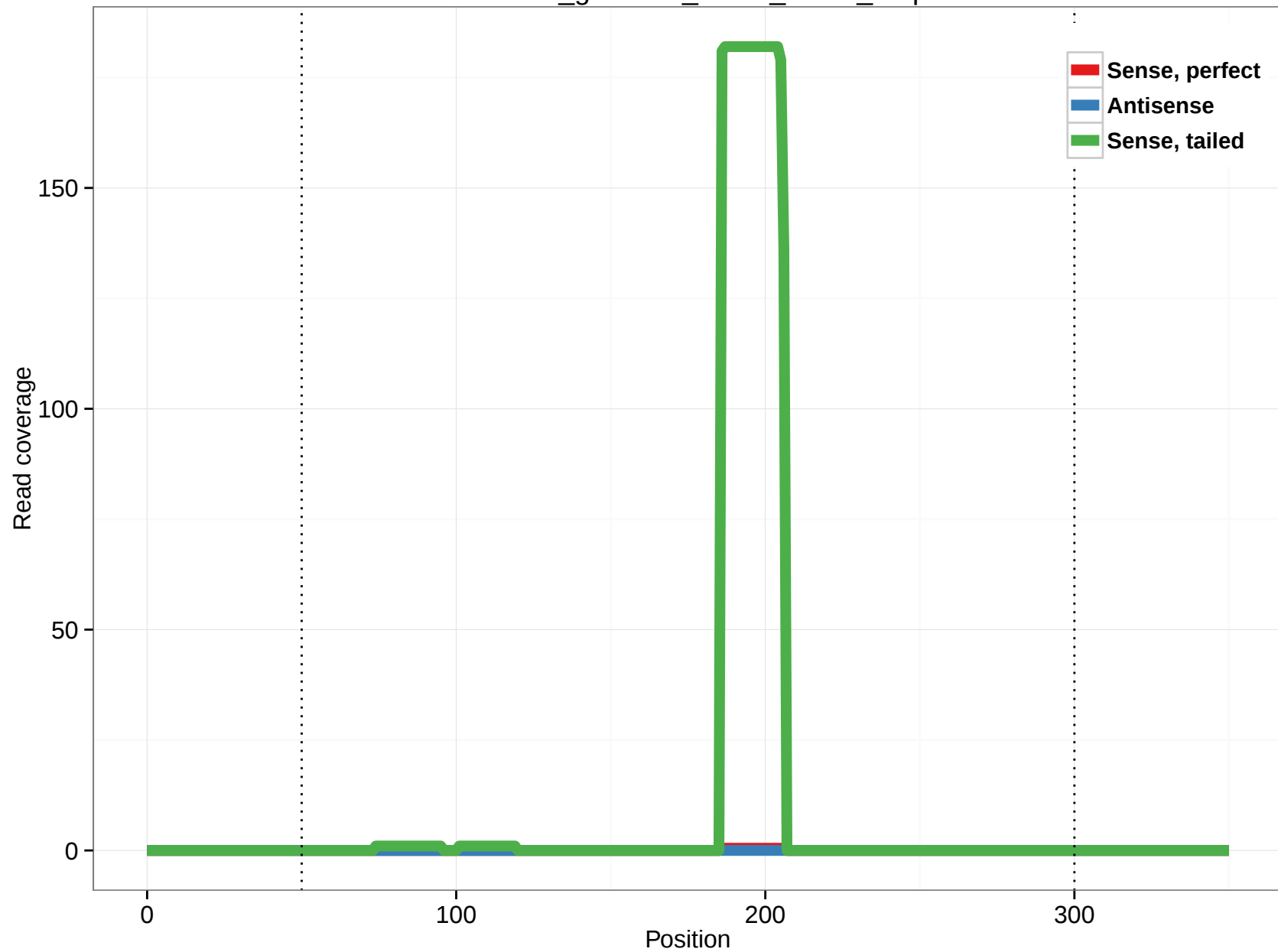
rheMac3_genscan_chr13_21.48_1.3p
