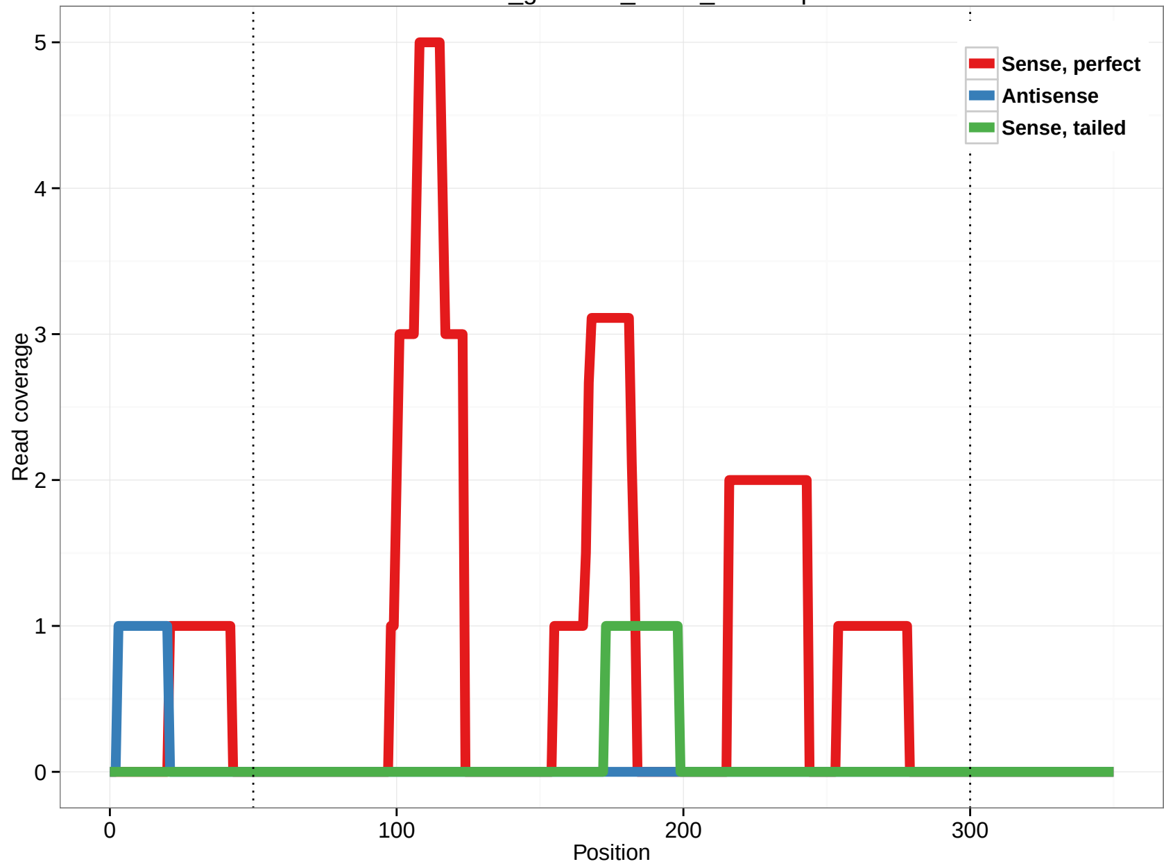
rheMac3_genscan_chr13_21.23.5p
