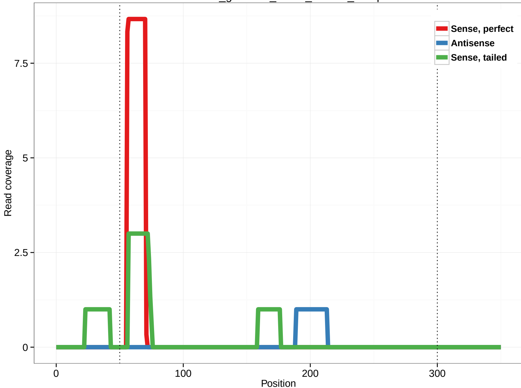
rheMac3_genscan_chr13_208.14_20.5p
