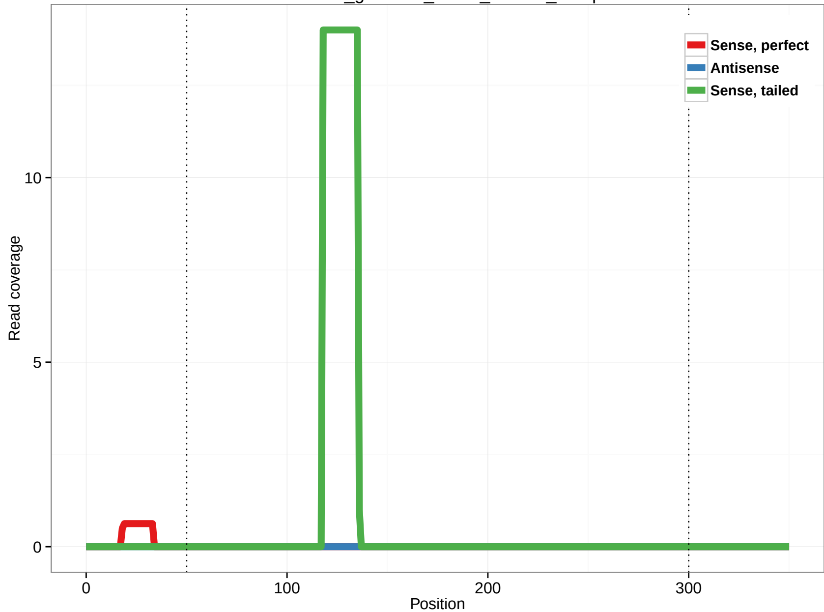
rheMac3_genscan_chr13_208.14_10.5p
