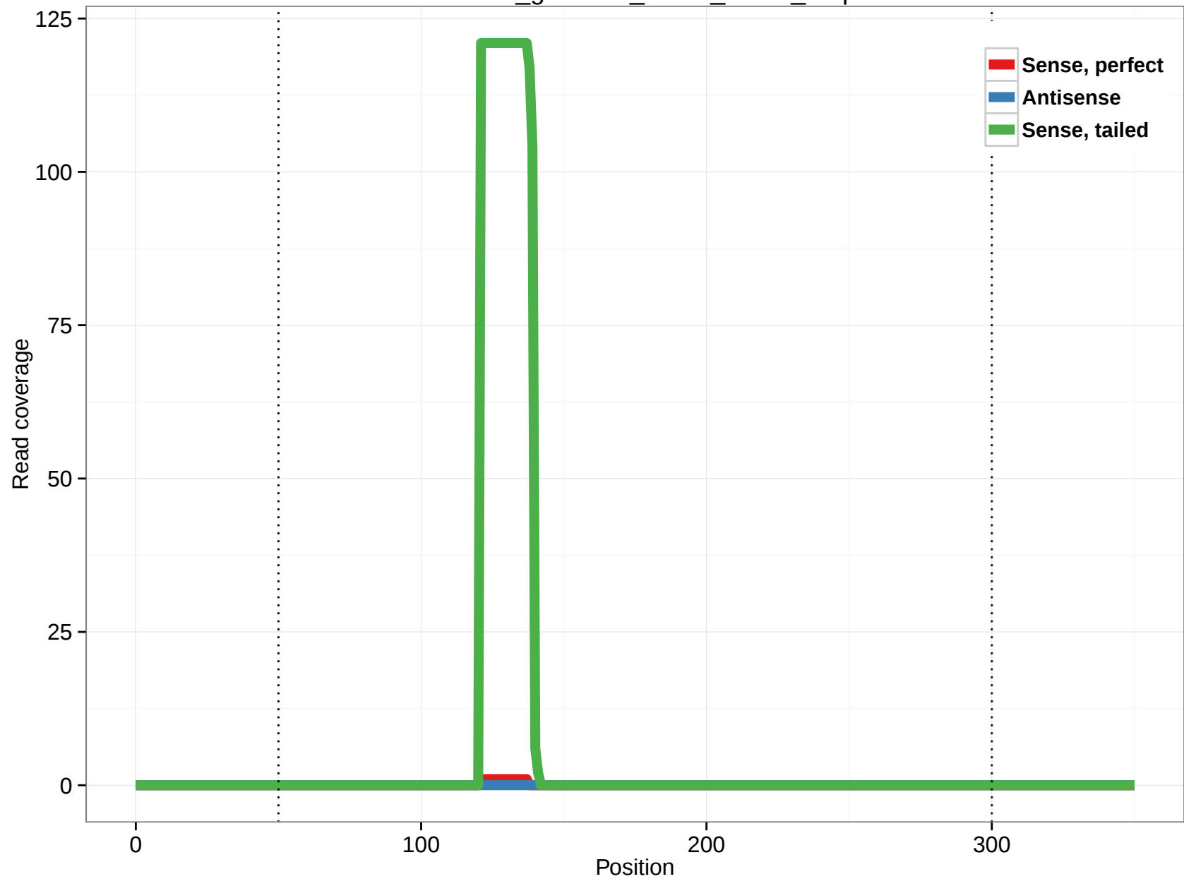
rheMac3_genscan_chr13_205.2_1.5p
