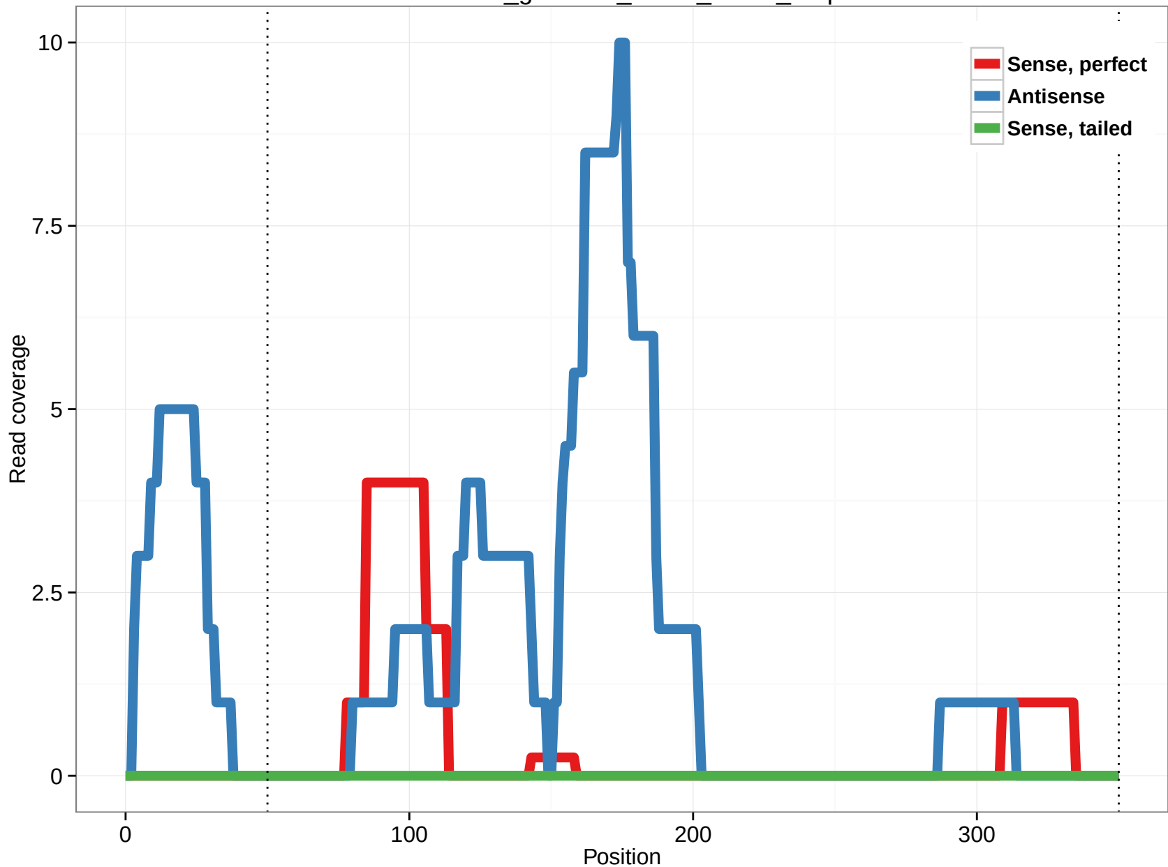
rheMac3_genscan_chr13_204.2_0.5p
