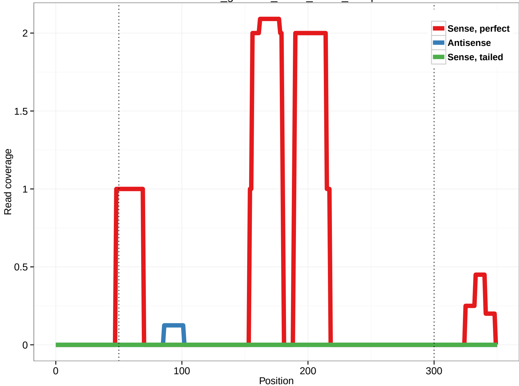
rheMac3_genscan_chr13_190.8_13.5p
