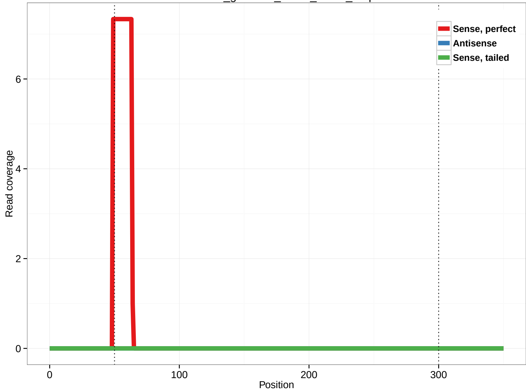
rheMac3_genscan_chr13_15.14_0.5p
