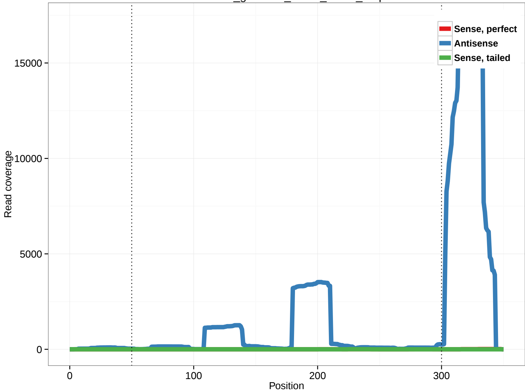
rheMac3_genscan_chr13_128.6_5.5p
