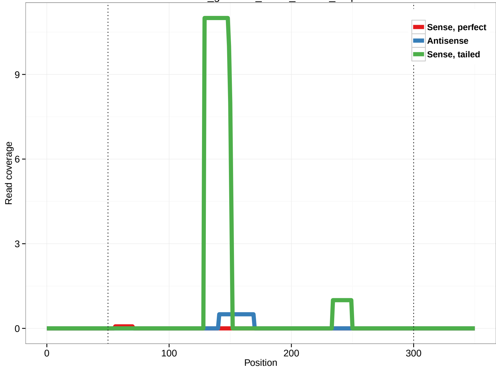
rheMac3_genscan_chr13_128.20_1.5p
