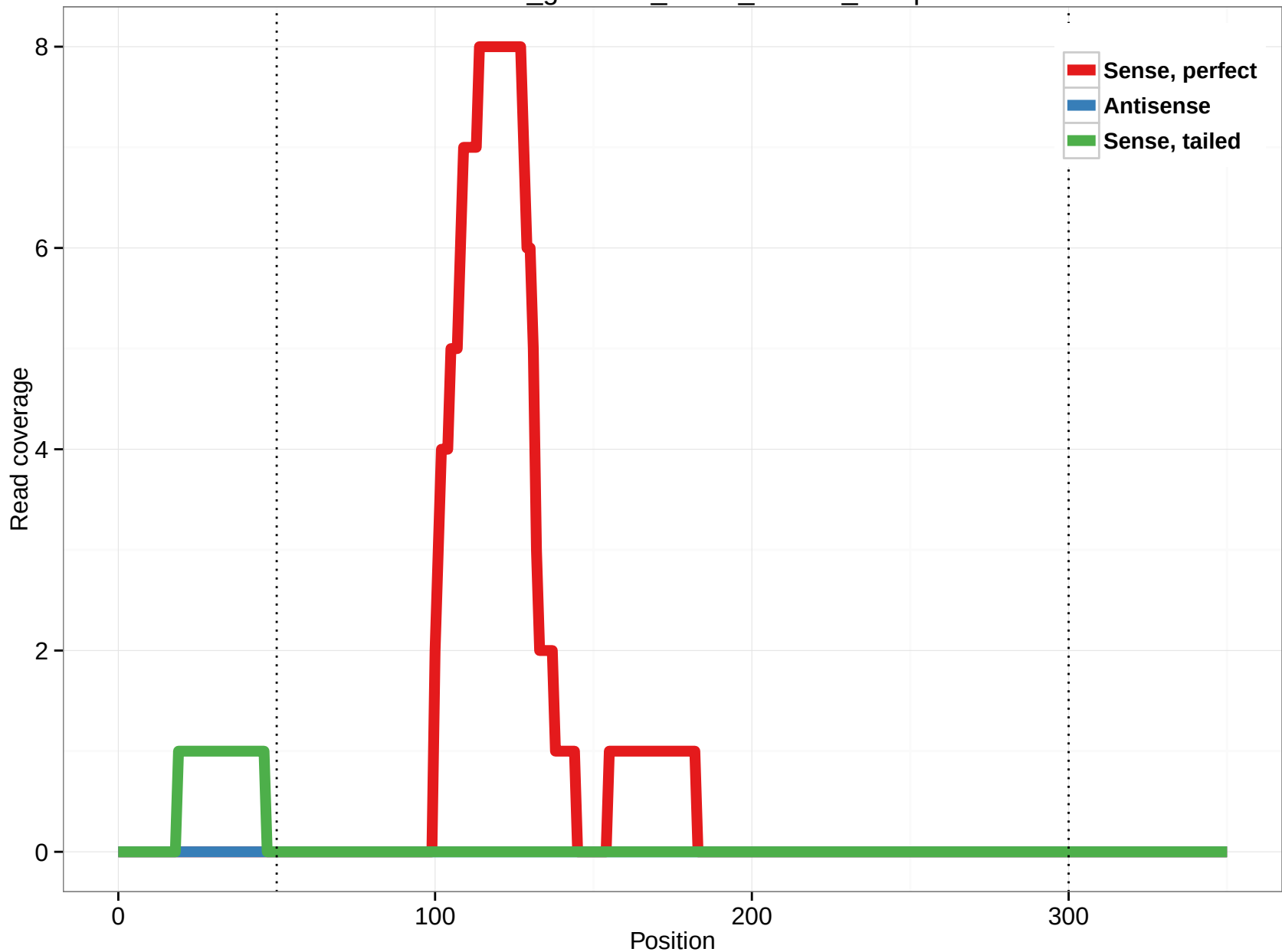
rheMac3_genscan_chr13_126.12_17.3p
