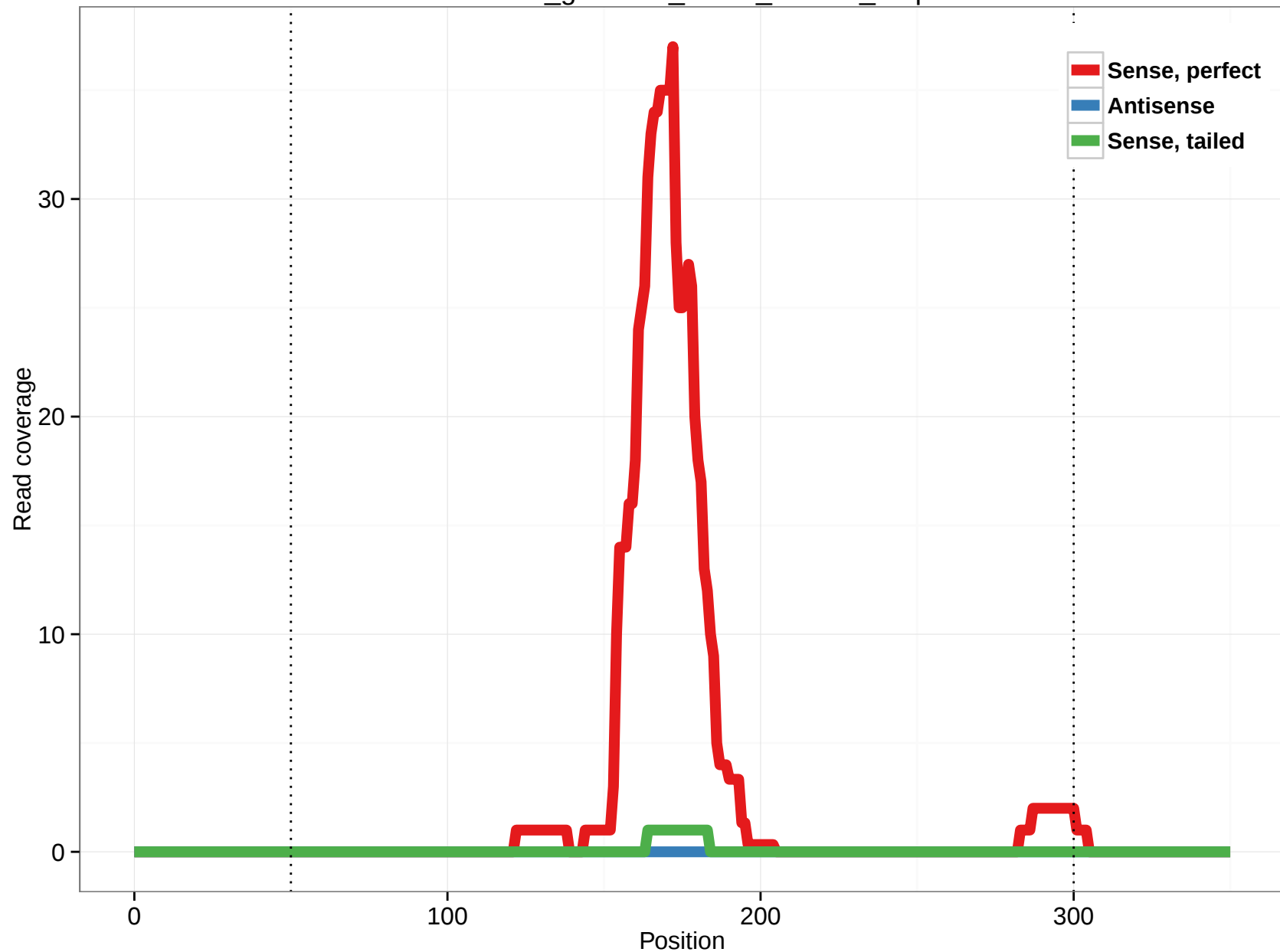
rheMac3_genscan_chr13_123.29_0.3p
