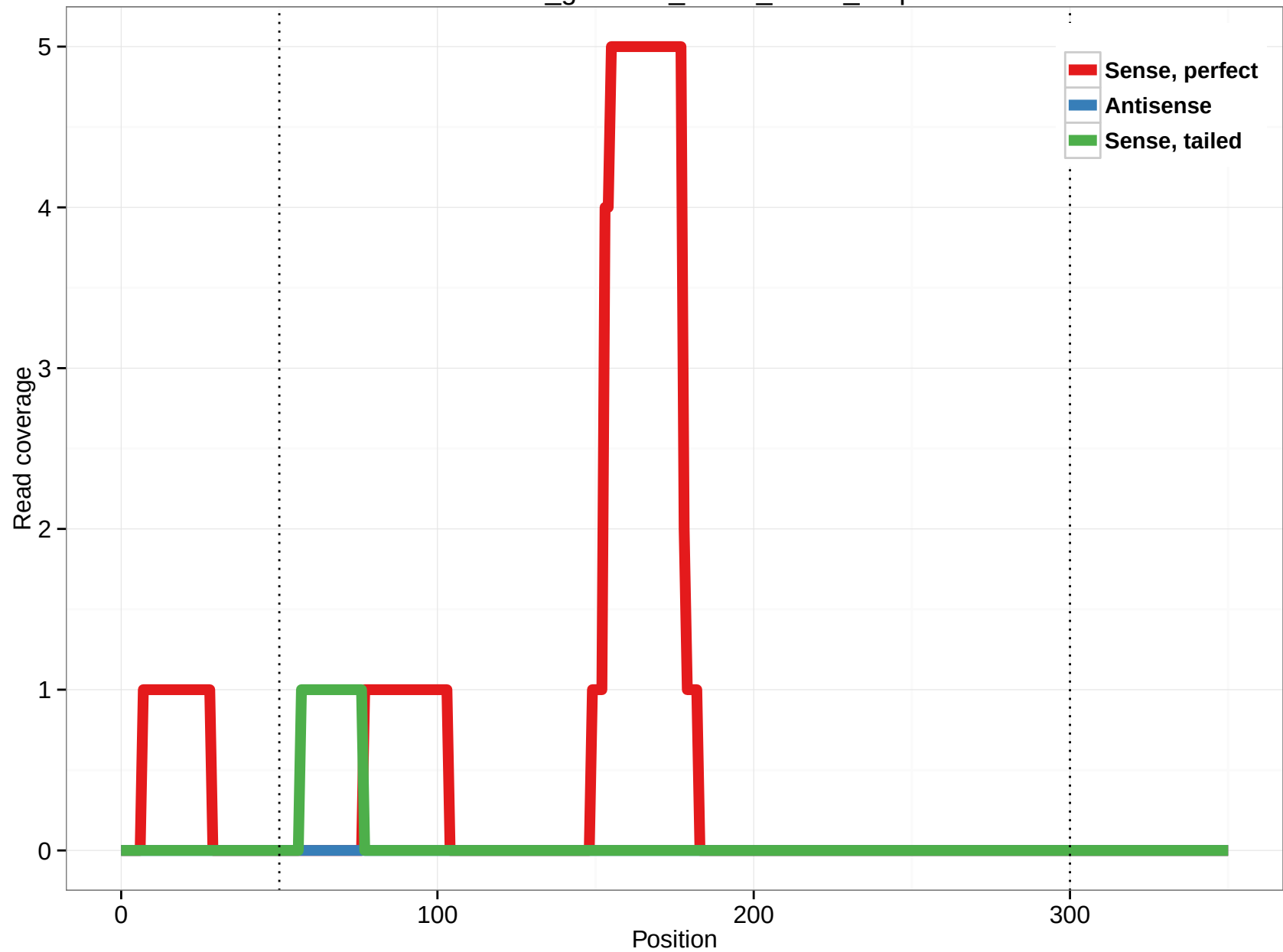
rheMac3_genscan_chr13_122.7_0.5p
