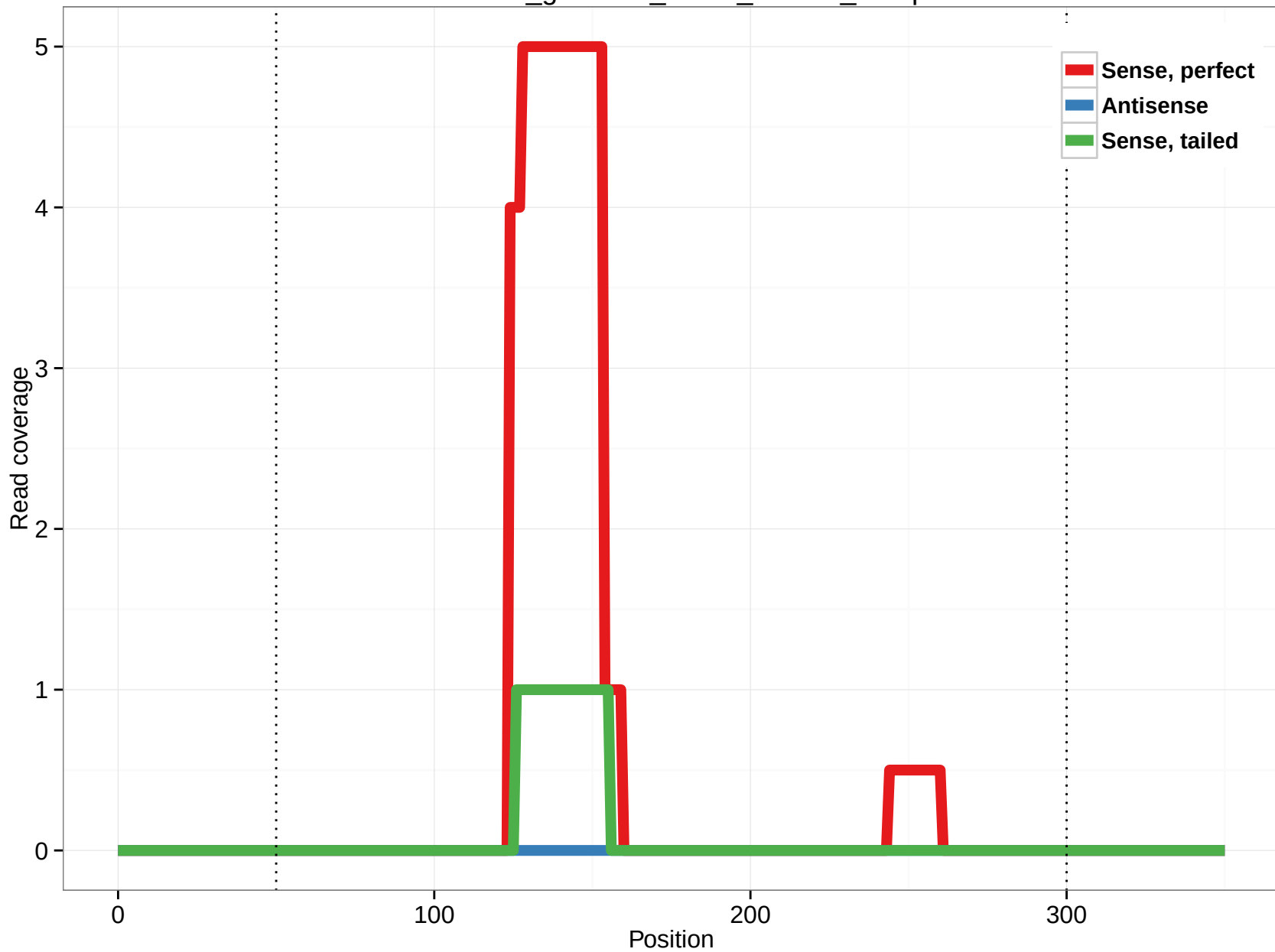
rheMac3_genscan_chr13_122.11_31.3p
