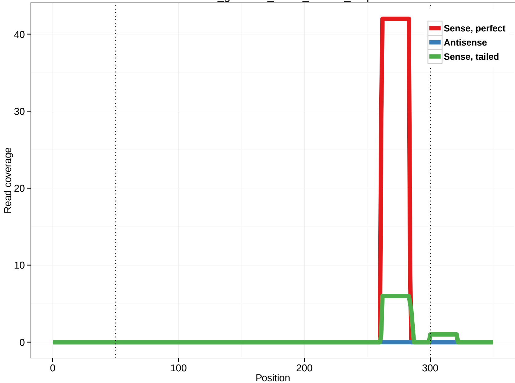
rheMac3_genscan_chr13_119.11_3.3p
