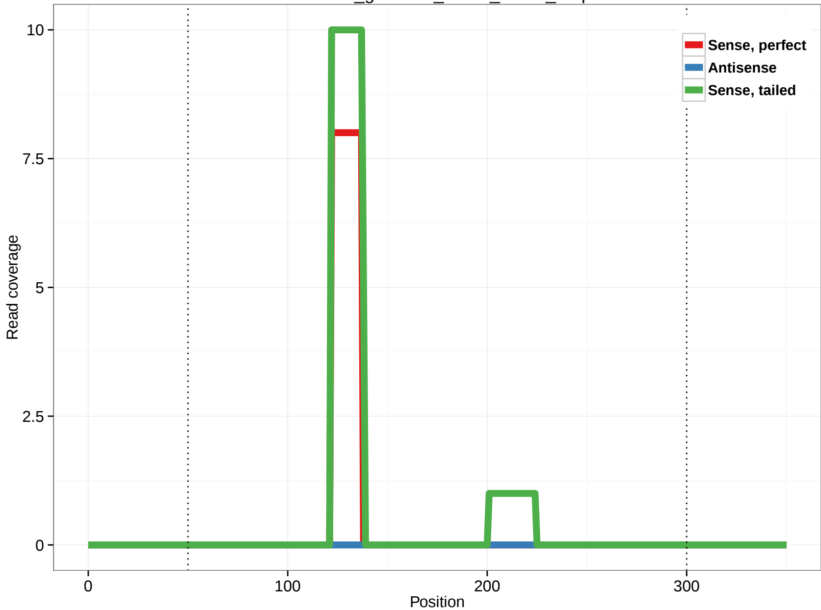
rheMac3_genscan_chr13_112.9_2.3p
