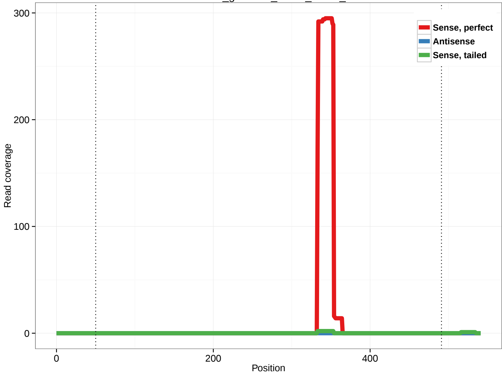
rheMac3_genscan_chr13_110.1_20
