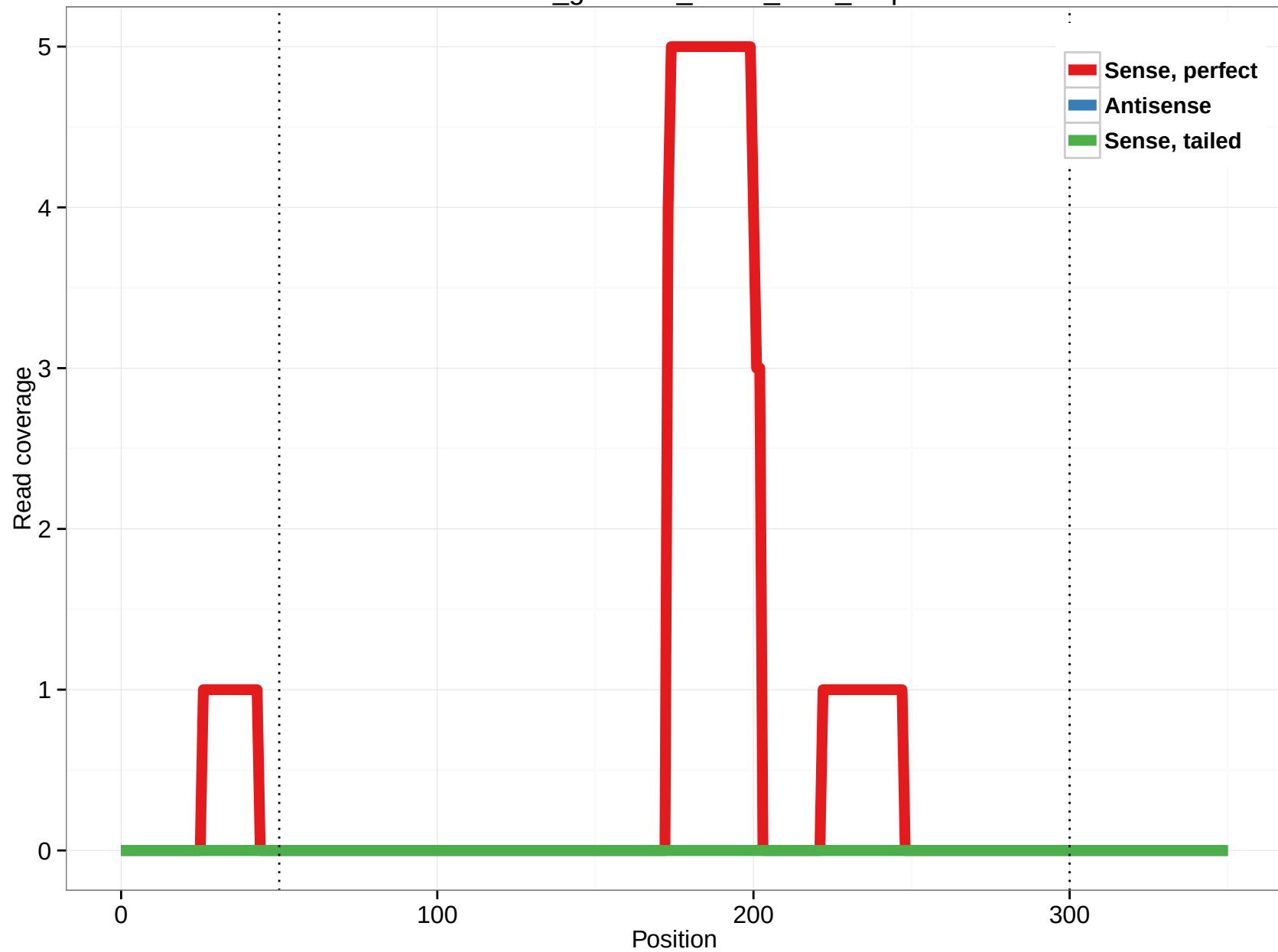
rheMac3_genscan_chr13_11.5_1.5p
