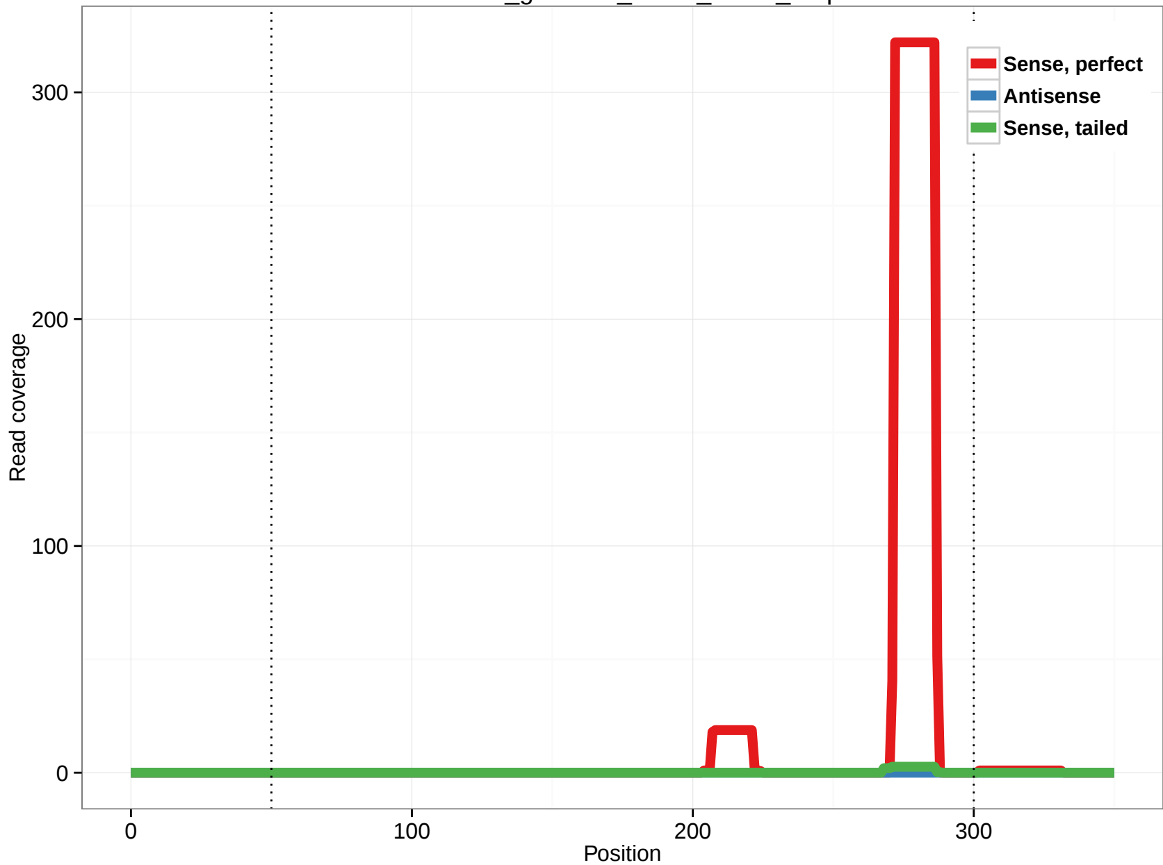
rheMac3_genscan_chr13_108.9_8.3p
