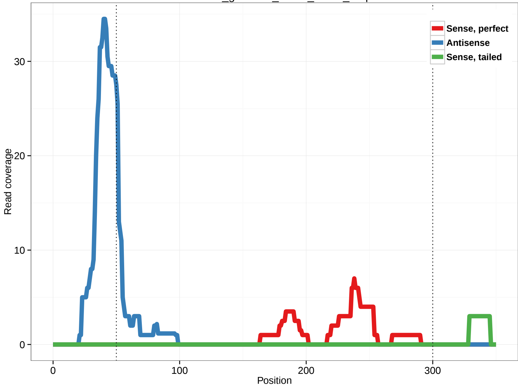
rheMac3_genscan_chr13_108.3_1.5p
