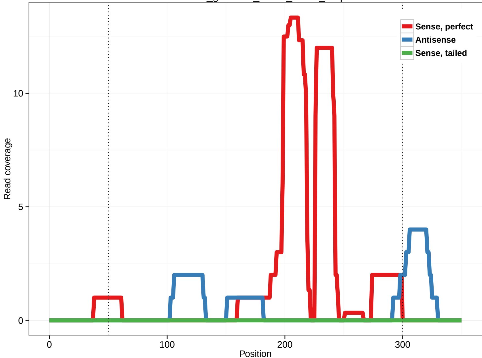
rheMac3_genscan_chr13_108.1_1.5p
