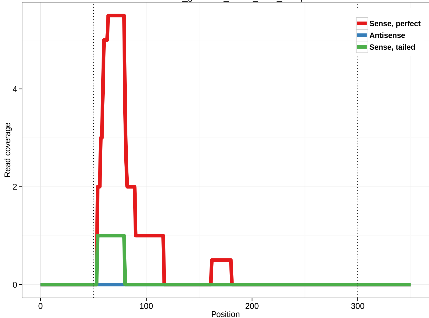
rheMac3_genscan_chr13_09.9_11.5p
