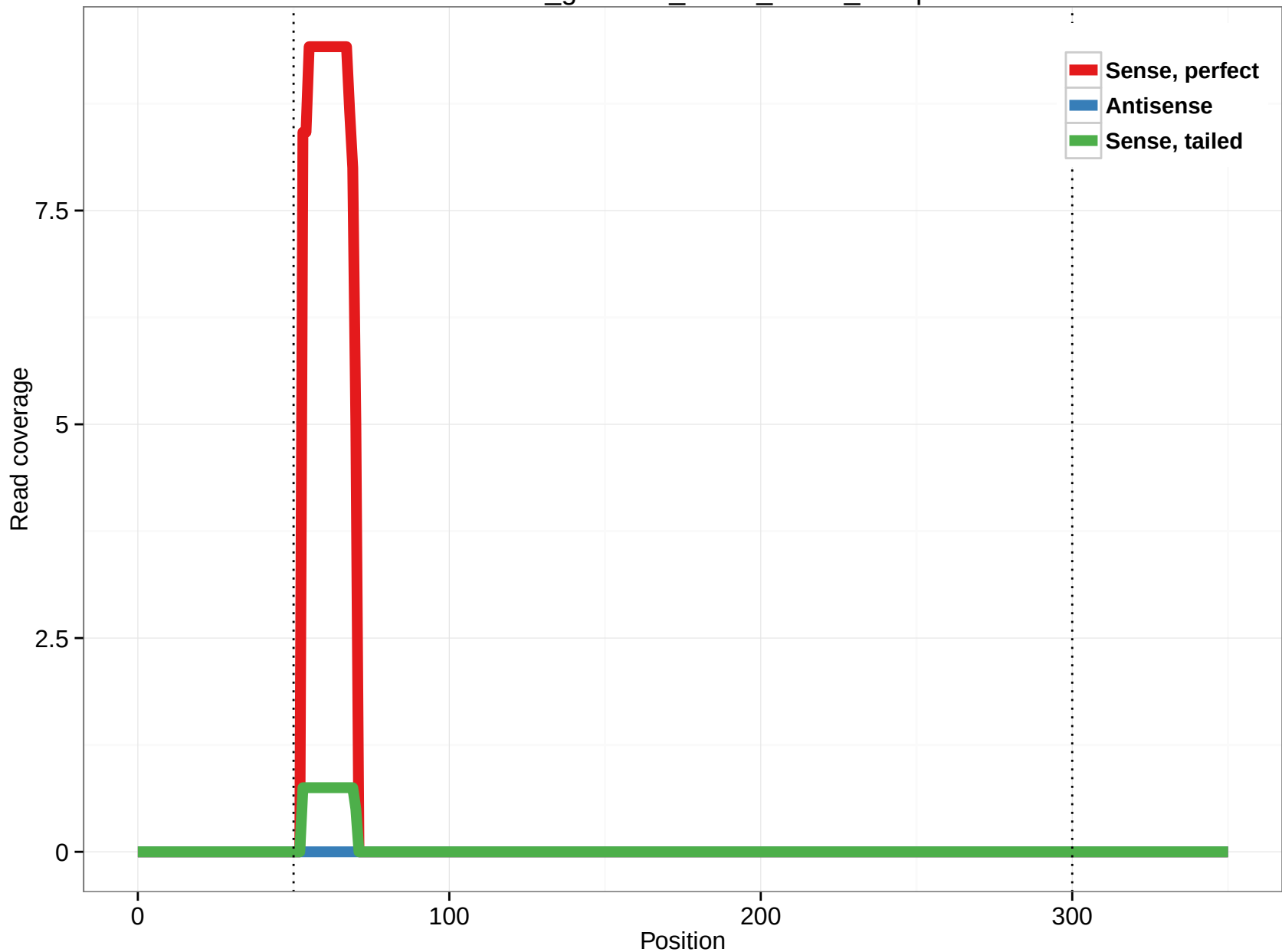
rheMac3_genscan_chr13_08.46_11.3p
