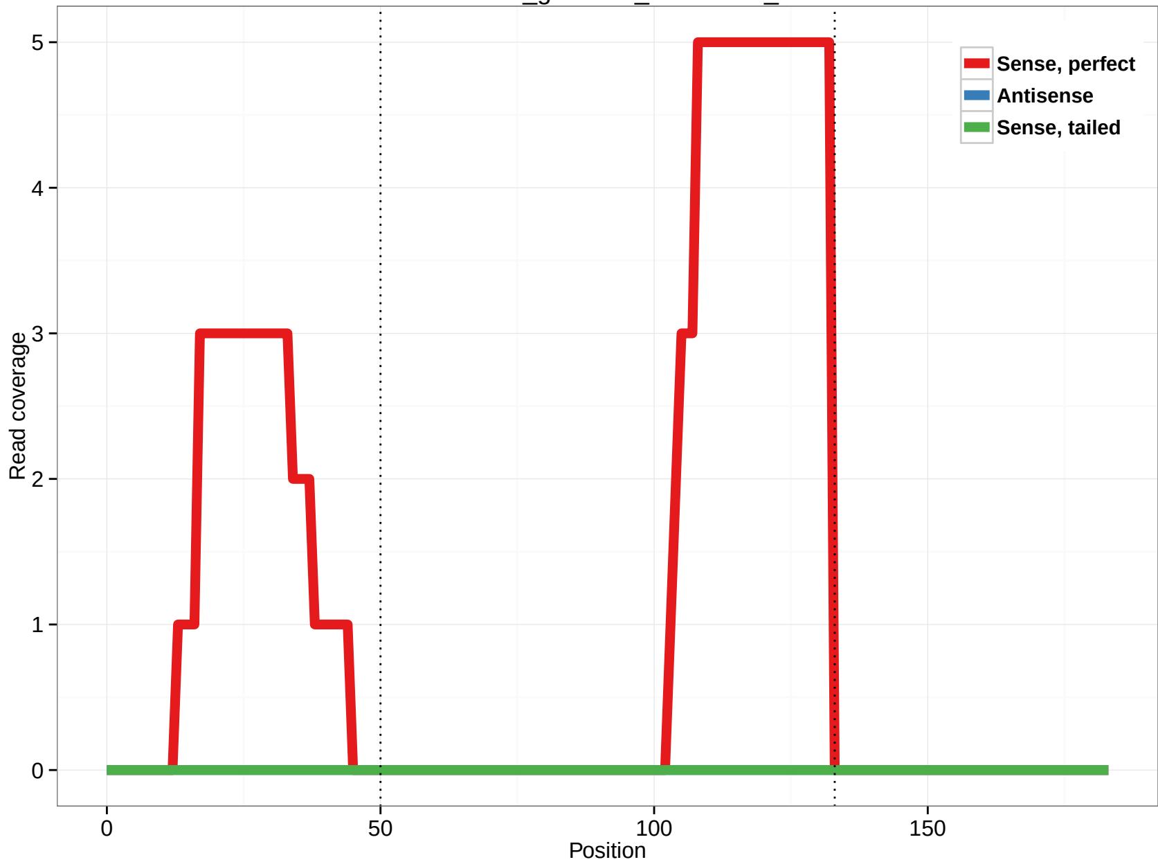
rheMac3_genscan_chr12.994_6
