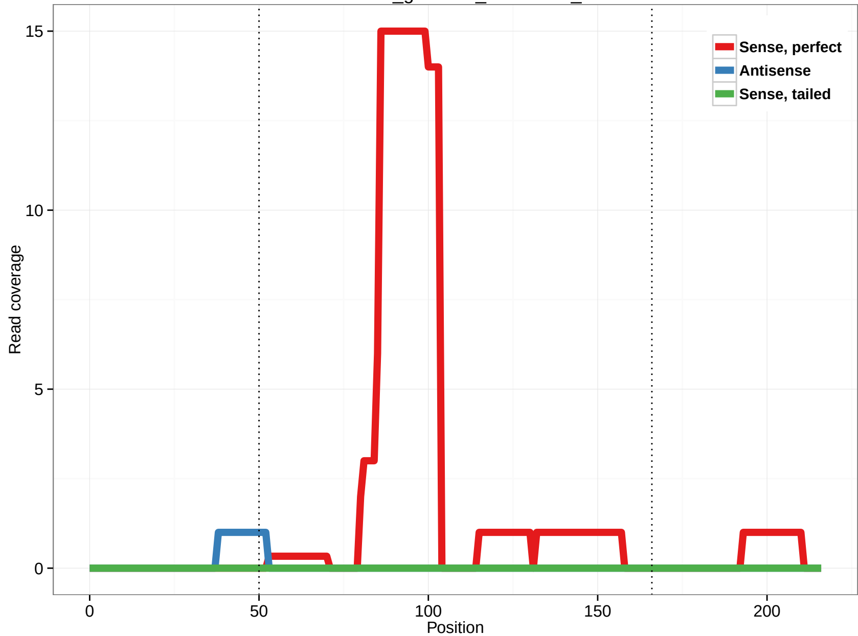
rheMac3_genscan_chr12.853_0
