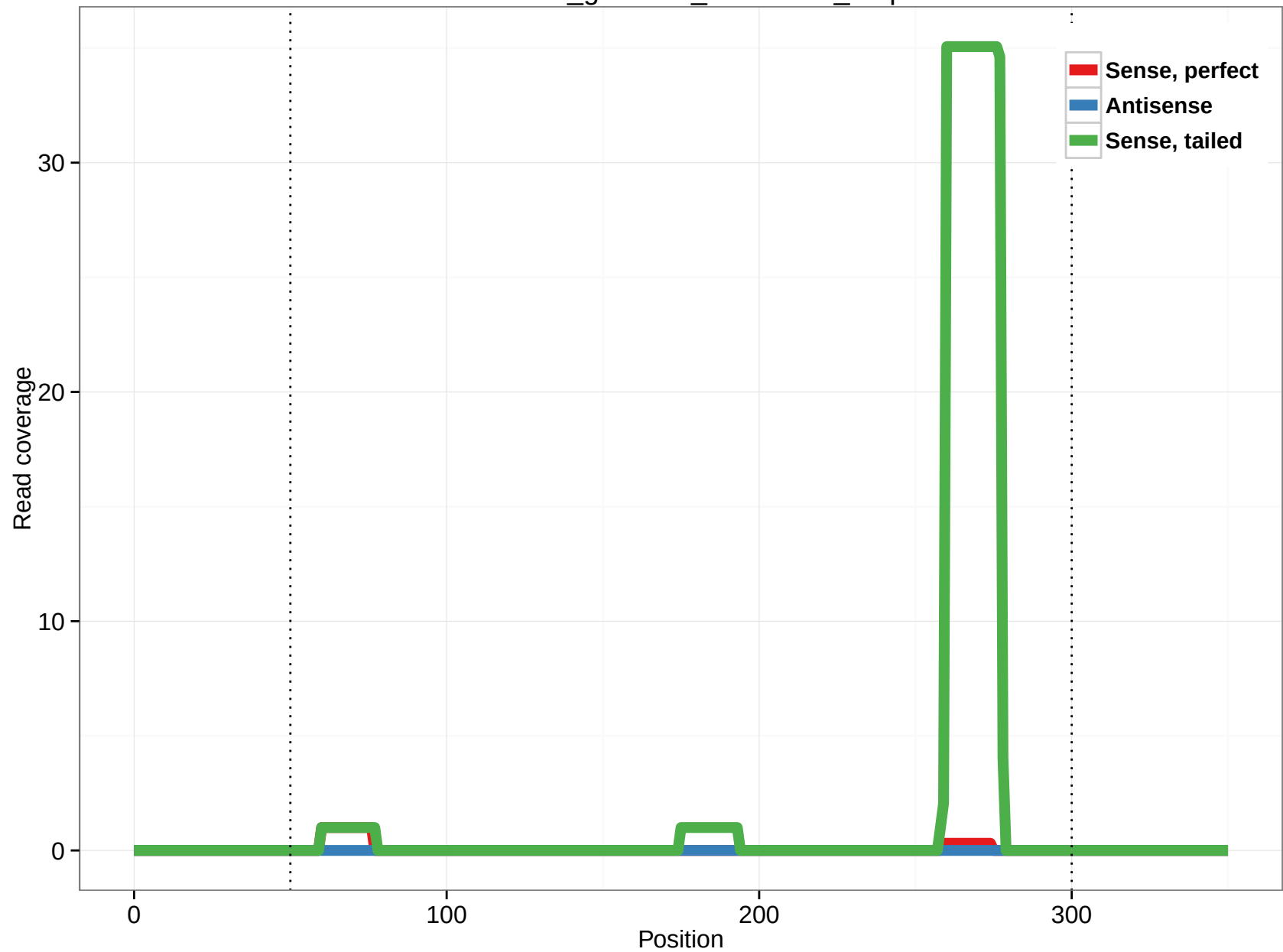
rheMac3_genscan_chr12.710_4.5p
