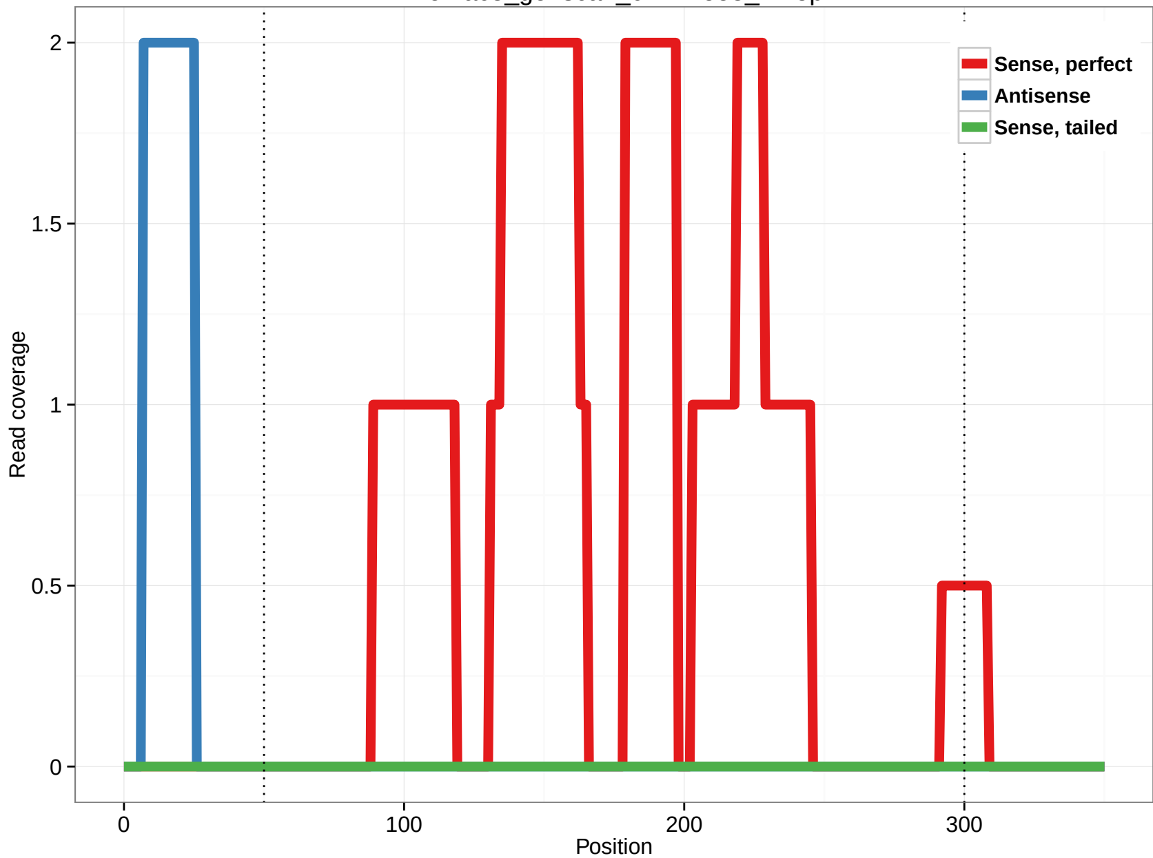
rheMac3_genscan_chr12.553_12.5p
