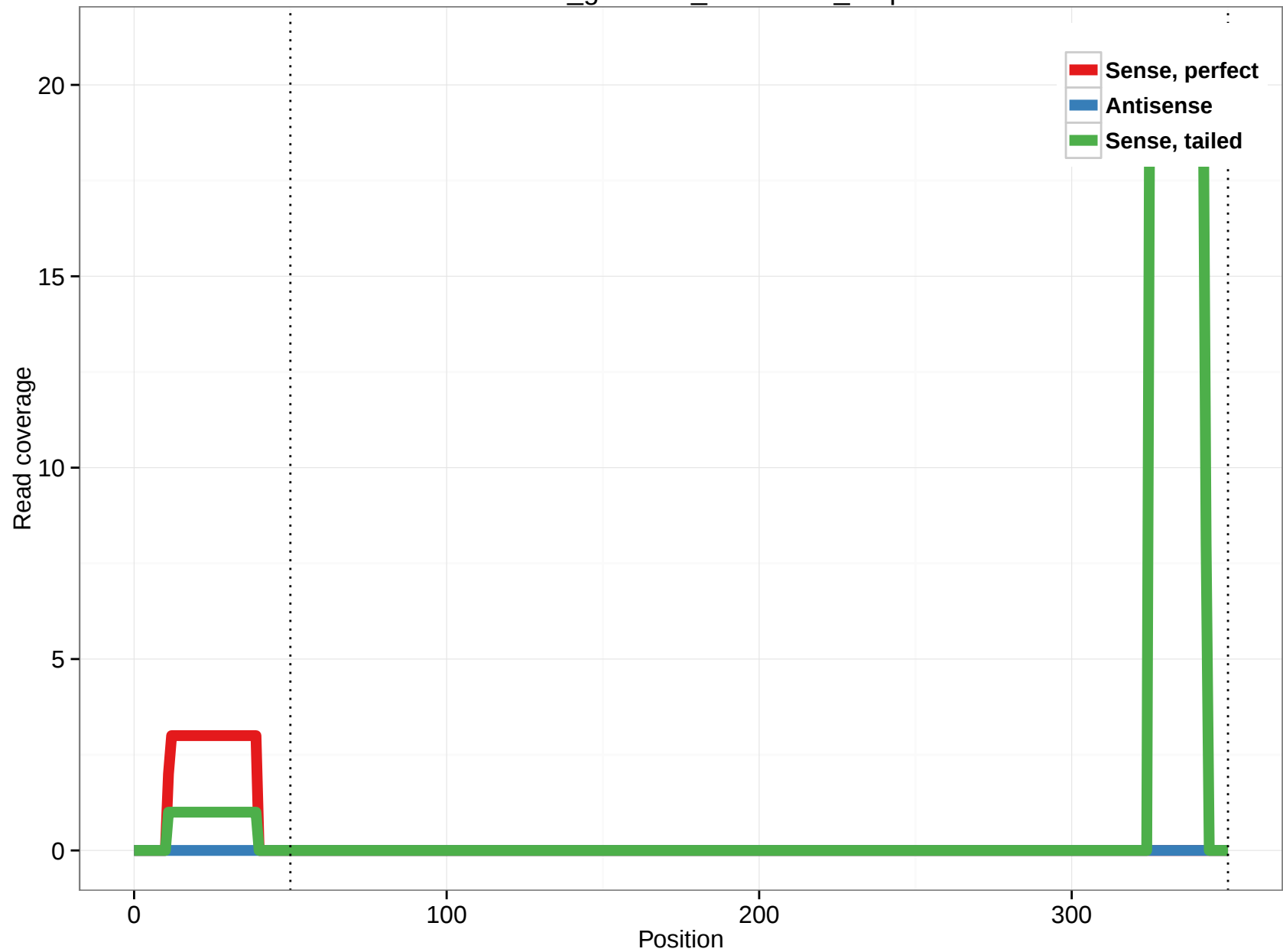
rheMac3_genscan_chr12.409_0.5p
