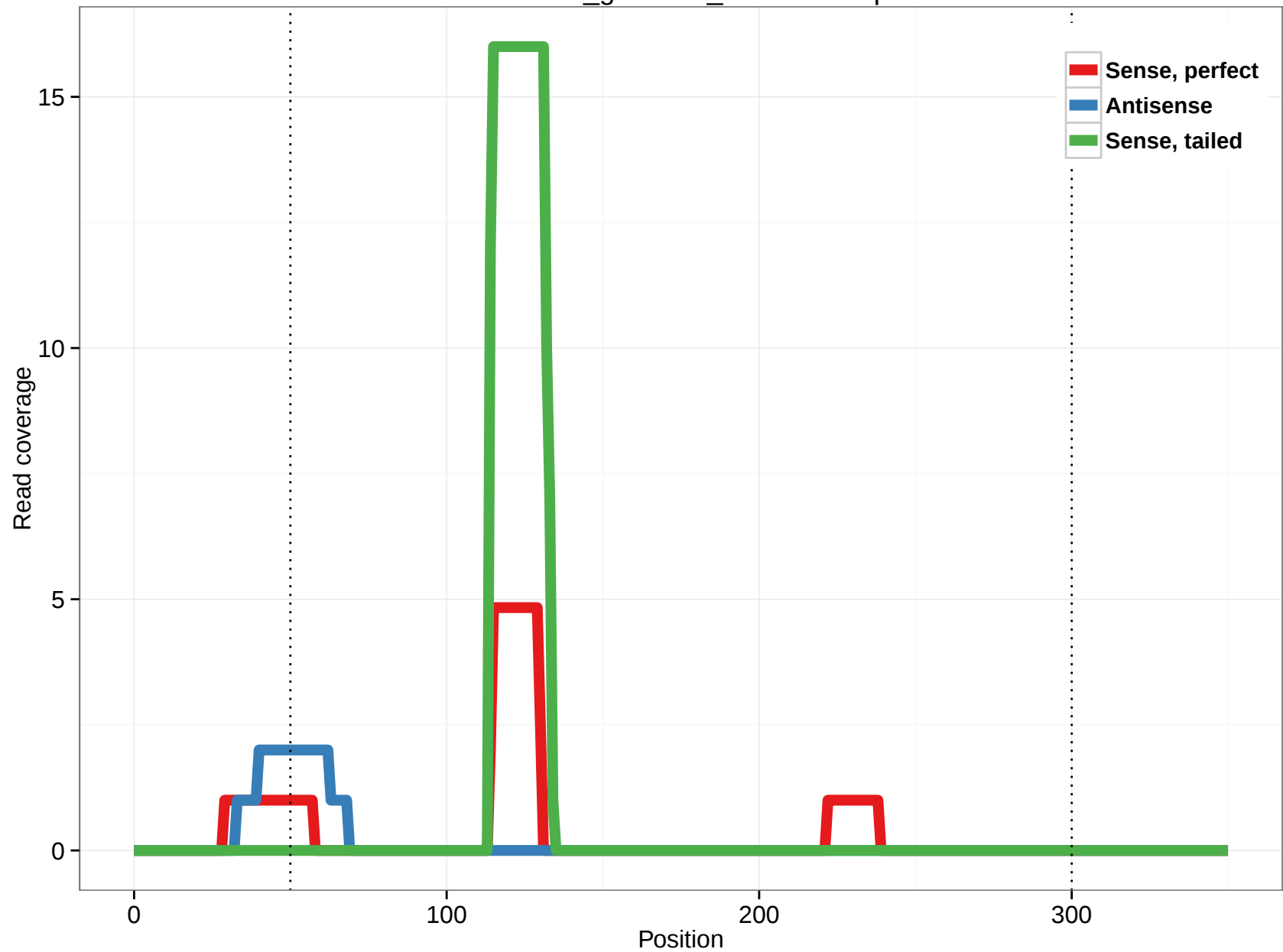
rheMac3_genscan_chr12.391.3p
