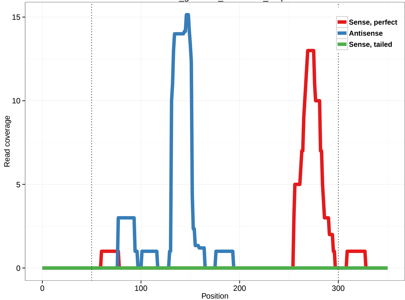
rheMac3_genscan_chr12.348_6.3p
