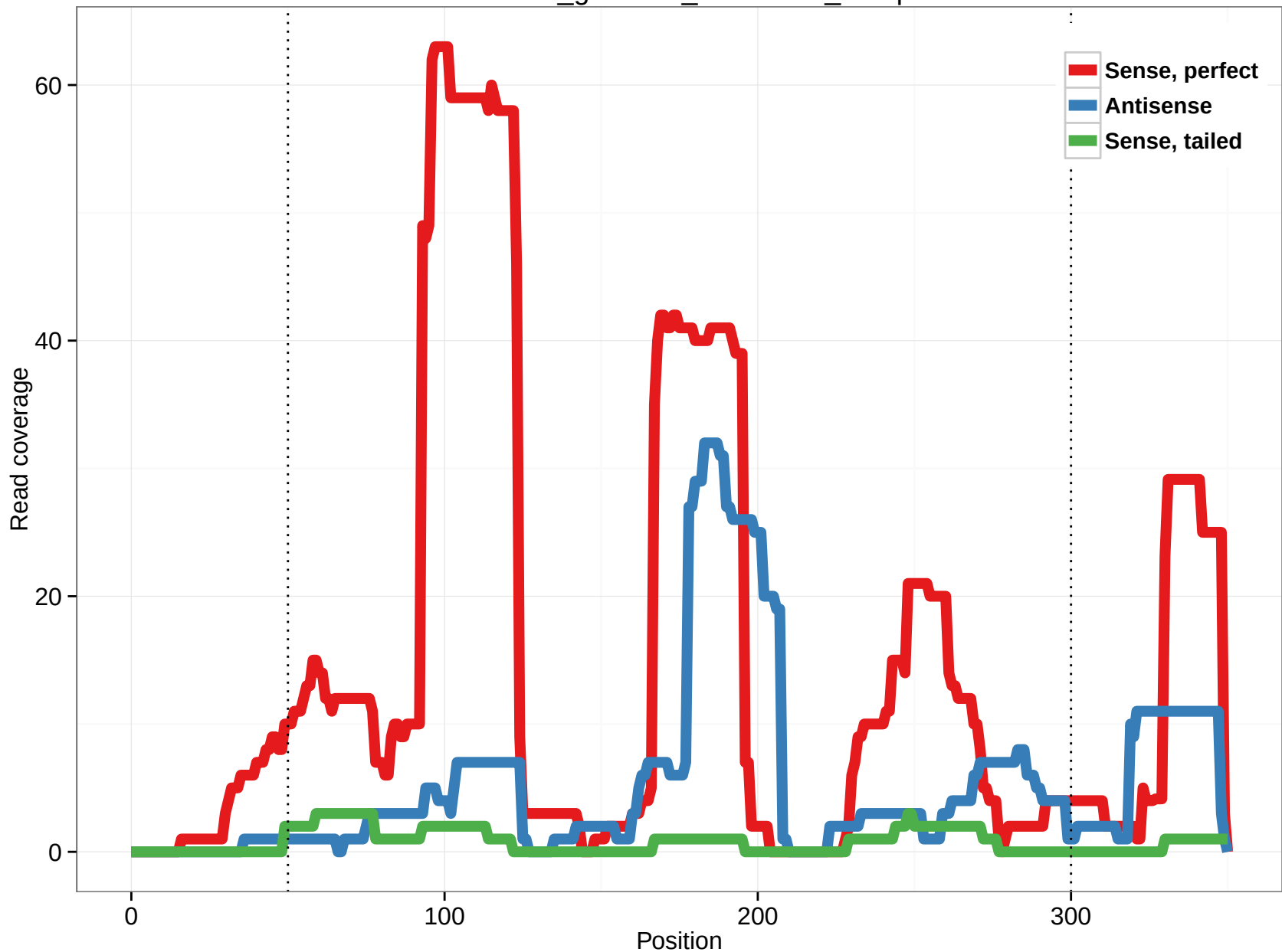
rheMac3_genscan_chr12.338_13.3p
