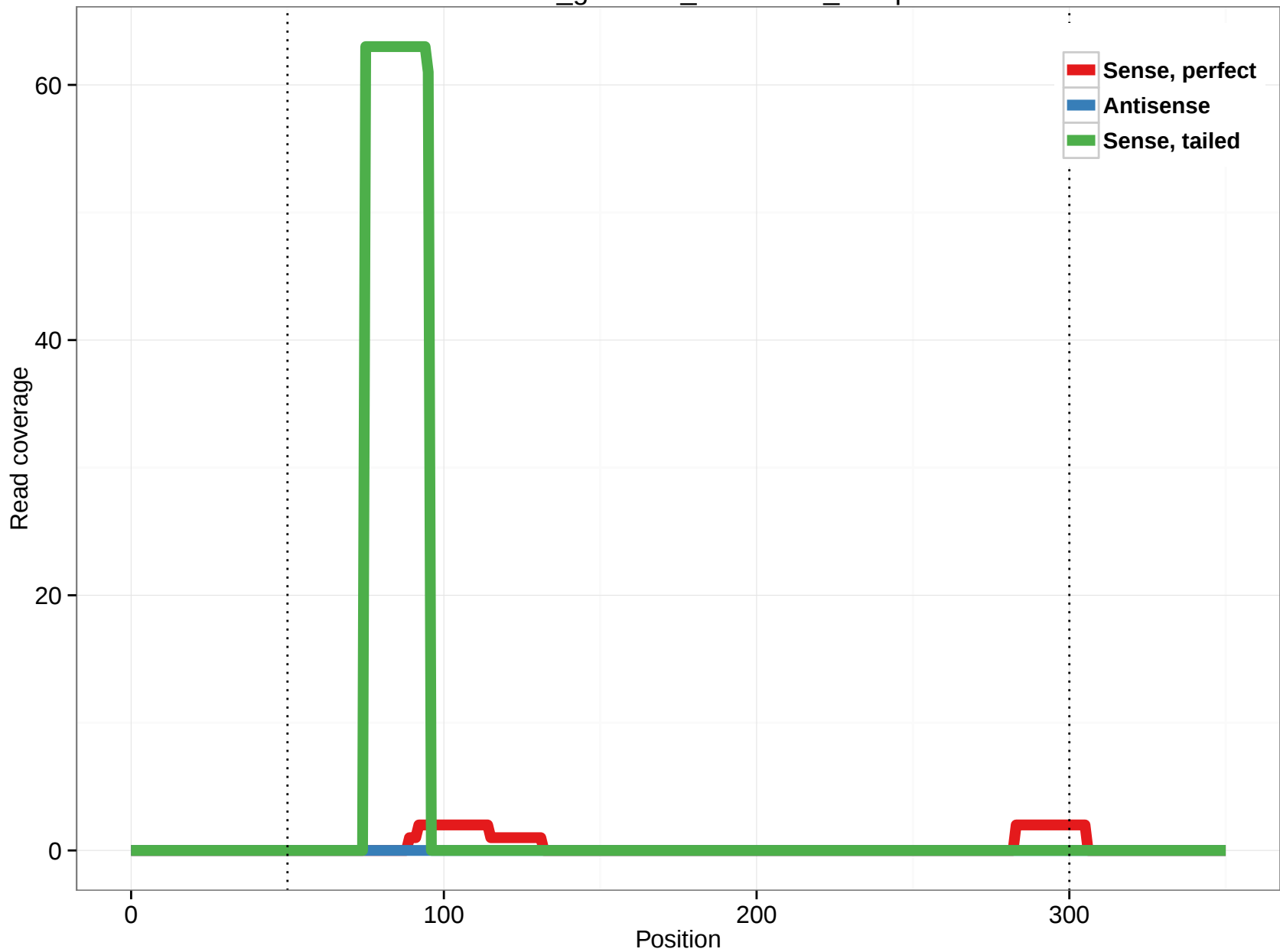
rheMac3_genscan_chr12.325_19.5p
